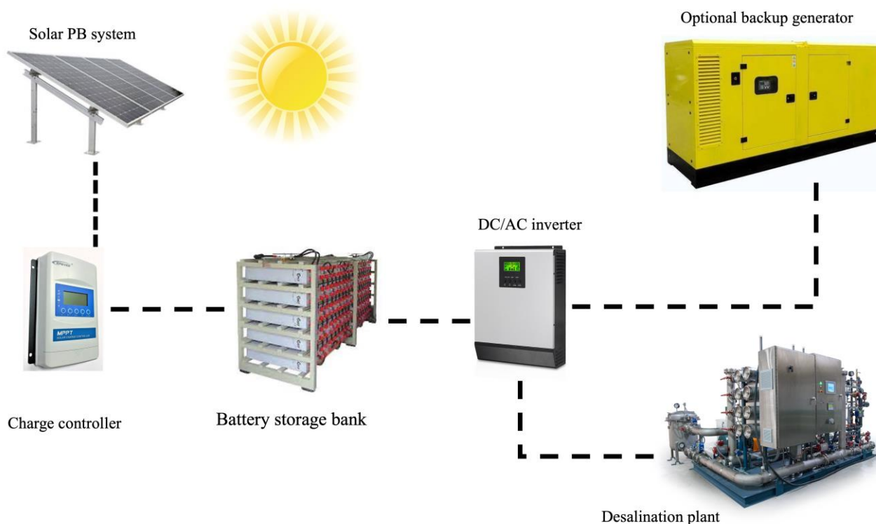
Figure 12. Schematic of solar water desalination system.
