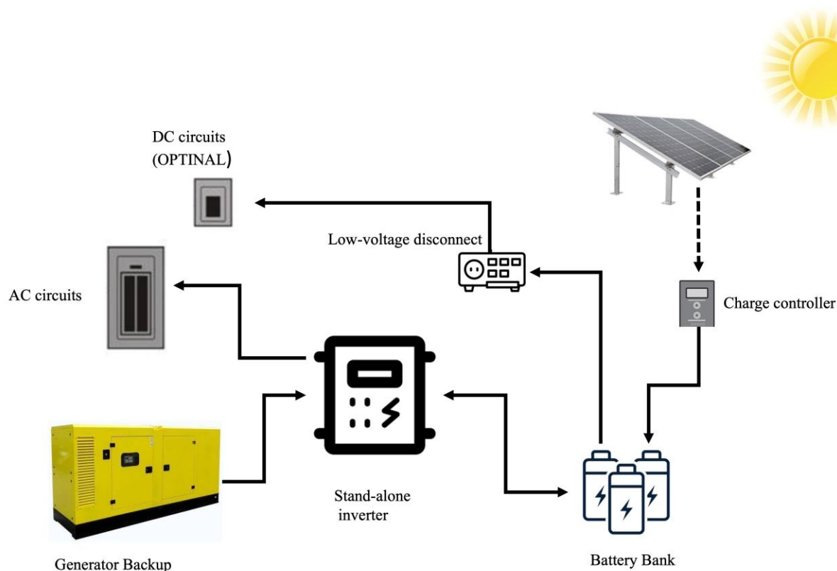
Figure 5. Rooftop stand-alone PV system with batteries.
