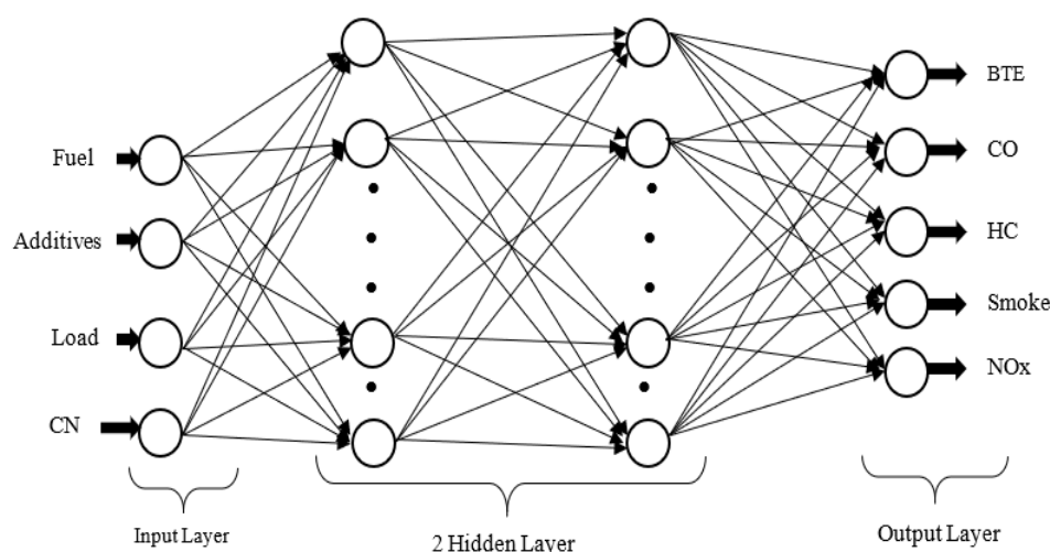
Figure 15. ANN Architecture.
