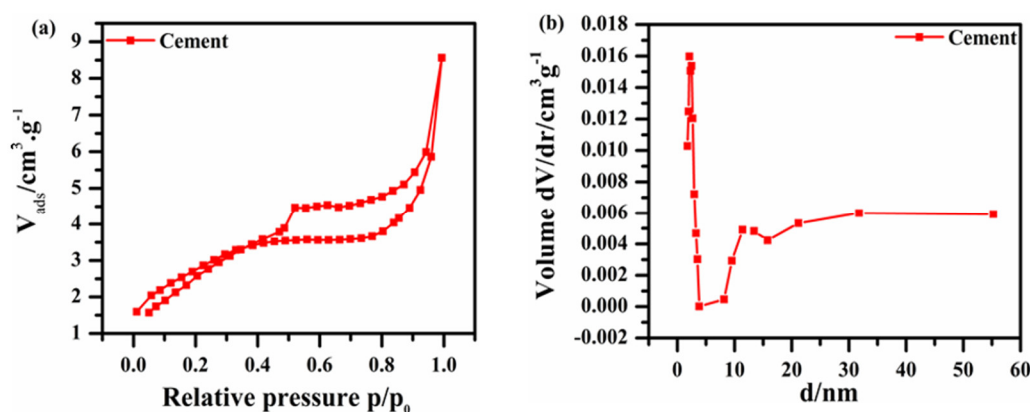
Figure 2. (a) The N 2 adsorption-desorption graphs at 77 K, and (b) the associated BJH pores diameter distribution rates for cement material.
