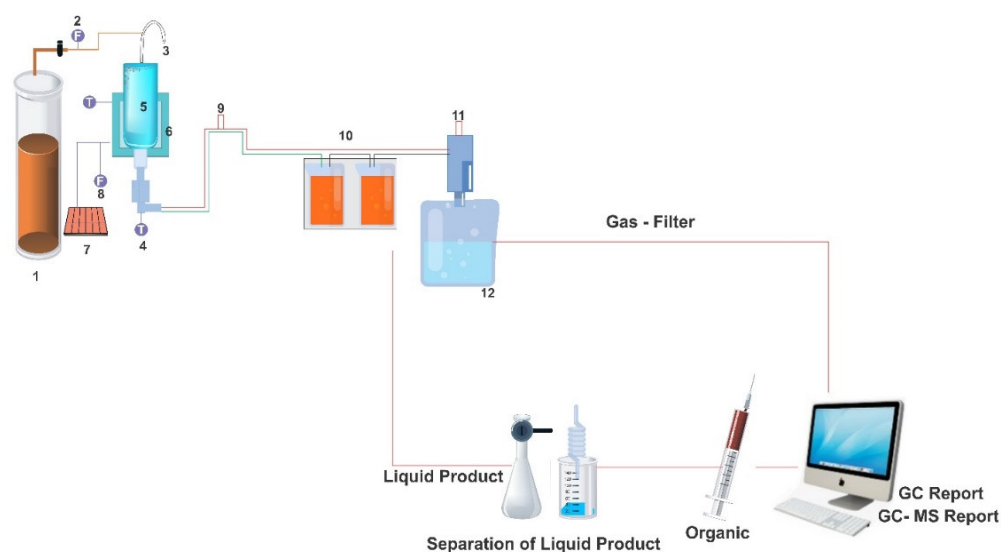
Figure 1. An illustration of the pyrolysis process in the bed reactor. Elements of the scheme: 1. N 2 container; 2. Flowmeter; 3. Exterior hook; 4. Thermo-couples; 5. Metallic tubes; 6. Thermal insulation; 7. Thermal regulator; 8. Electrical energy; 9. Air valves; 10. The air conditioning device; 11. Windbag, and 12. Gasbag.
