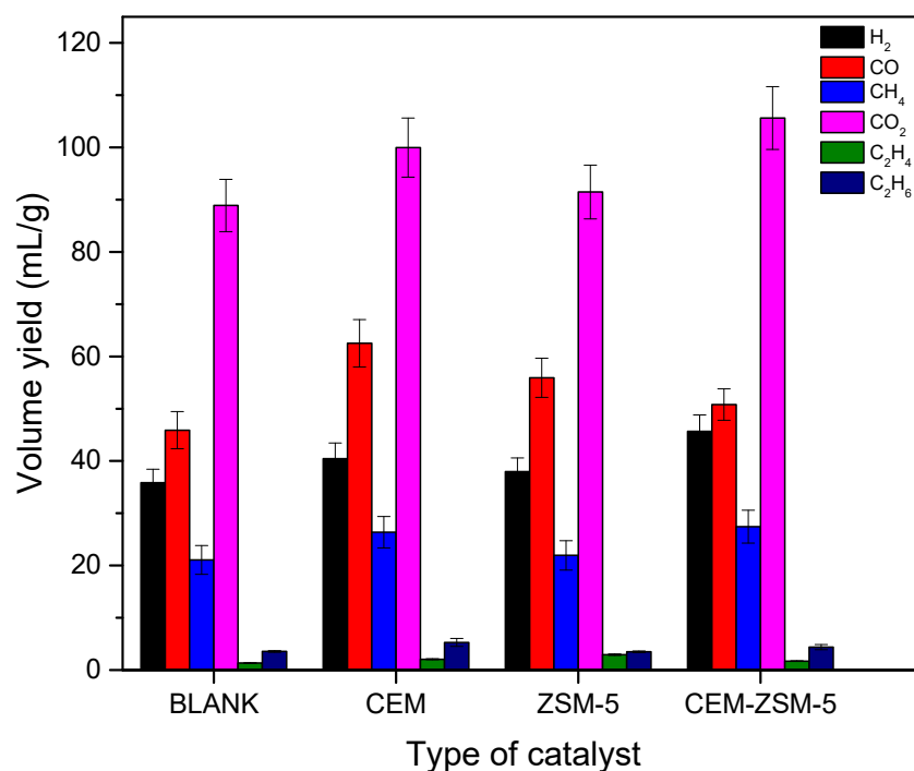
Figure 3. Impact of different catalysts on gas volume output at 600 °C taking the reaction blank as reference (Data collected in Table S1).
