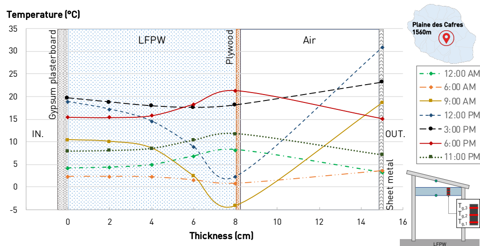
Figure 13. Evolution of the thermal gradient of the ceiling during the day with the widest day/night range (2 September 2020).
