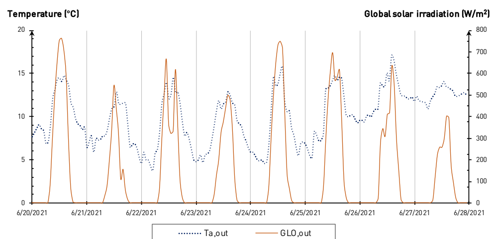
Figure 8. Evolution of meteorological parameters T_{a,out} and GLO_{out} during the coldest week of the second part of the measurement period.
