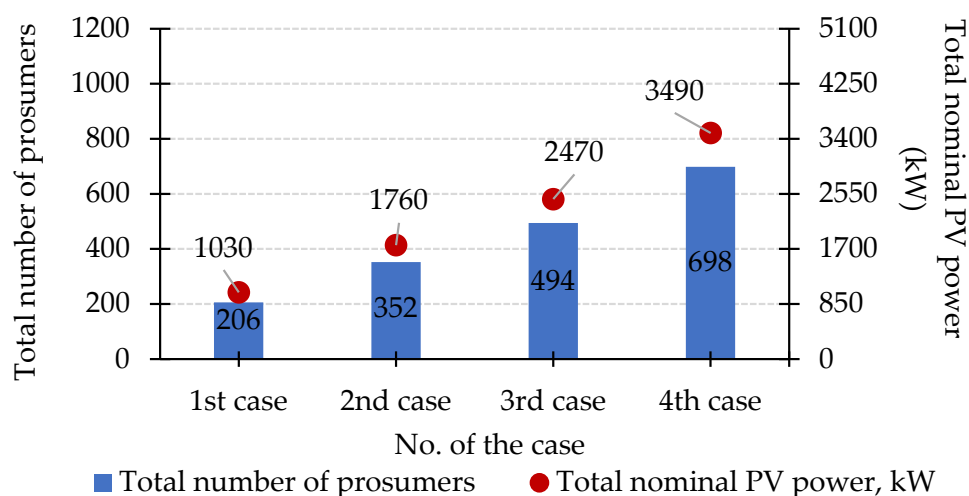
Figure 4. The total capacity of PV installations and the total number of prosumers by case number.
