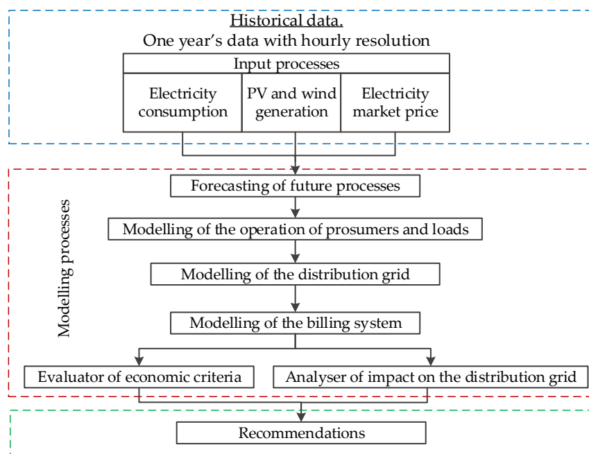
Figure 2. The structure of the decision-making algorithm.
