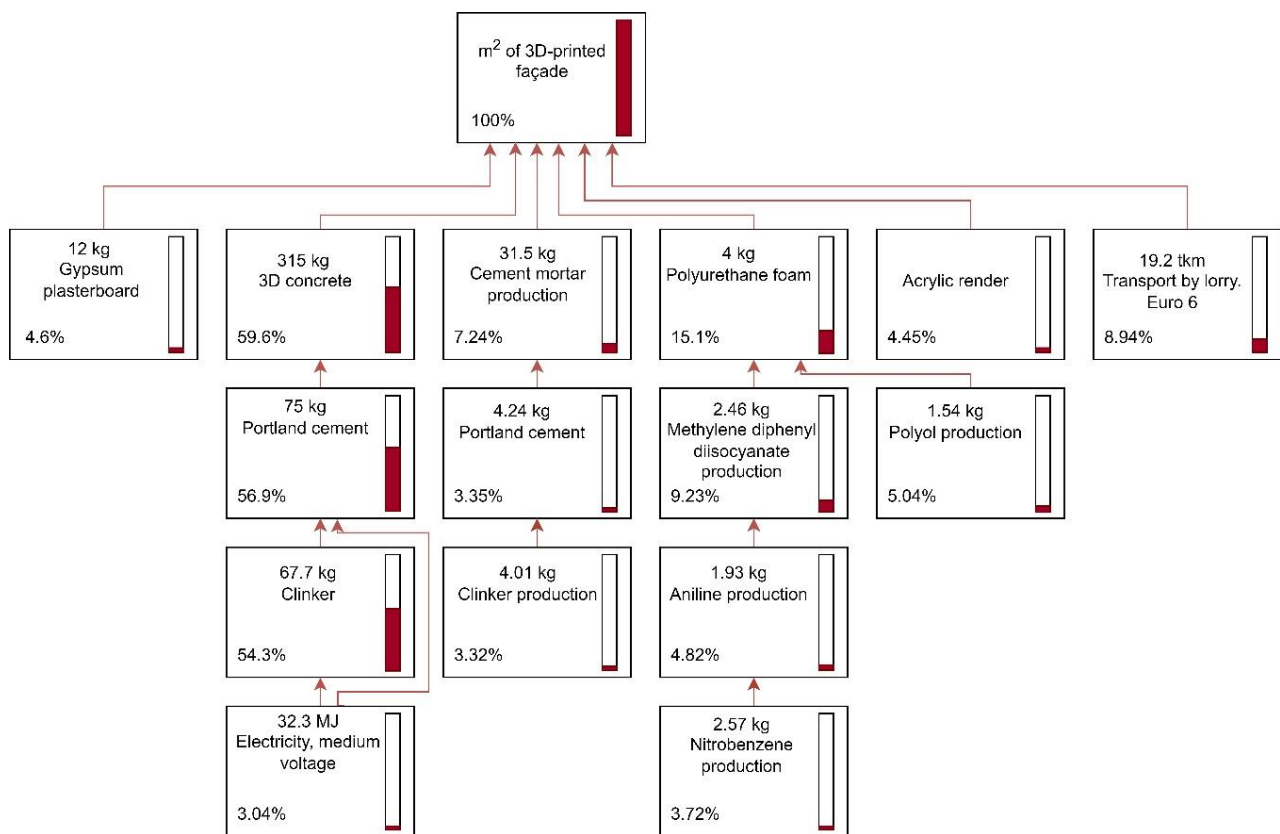
Figure 11. Contribution of each process of the 3D-printed façade to the total carbon emissions.
