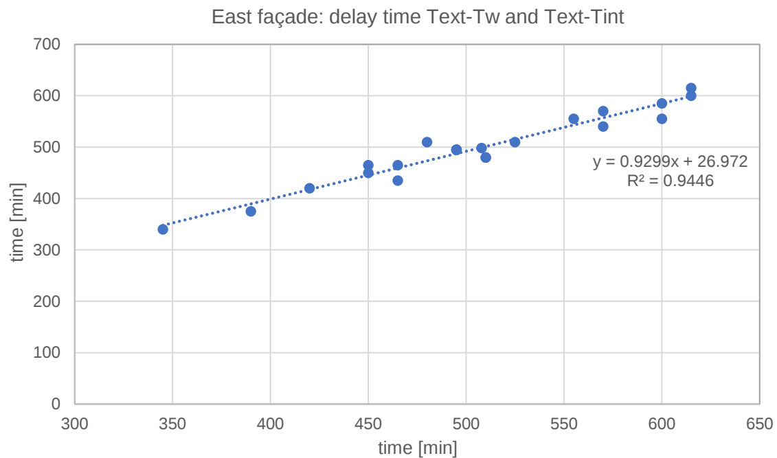
Figure 9. East façade: time lag between T_{ext} and T_w and T_{ext}-T_{int} dispersion.
