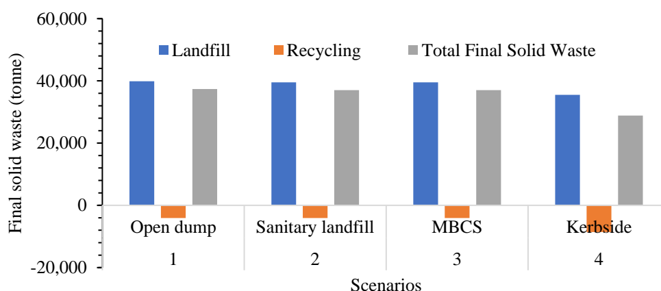
Figure 8. The final solid waste of the four scenarios.
