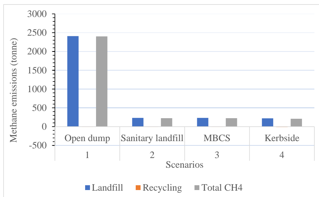
Figure 11. Methane emissions across all four scenarios.
