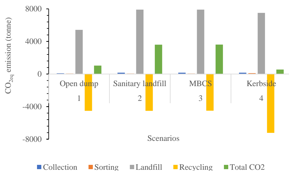
Figure 9. Comparative total CO 2eq emission (in ton) from all four scenarios.
