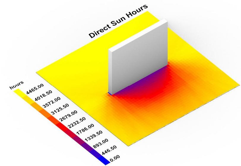
Figure 9. Sun hours analysis with Ladybug.
