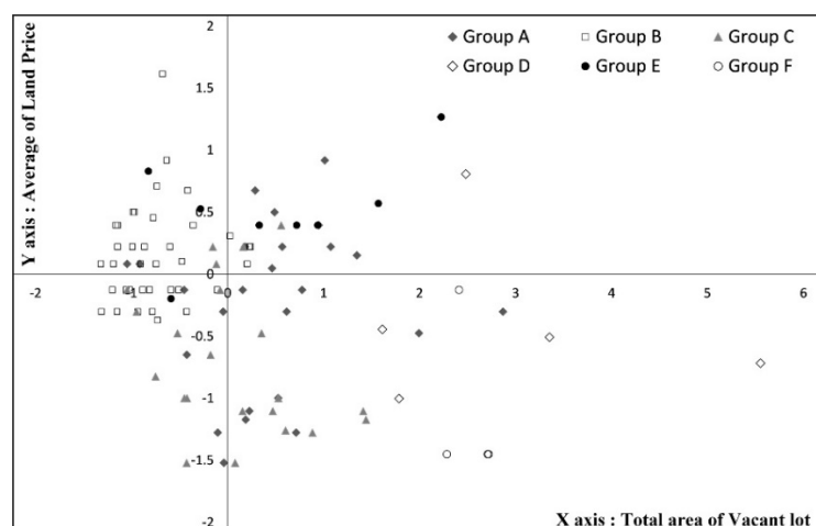
Figure 15. Scatter diagram (2).
