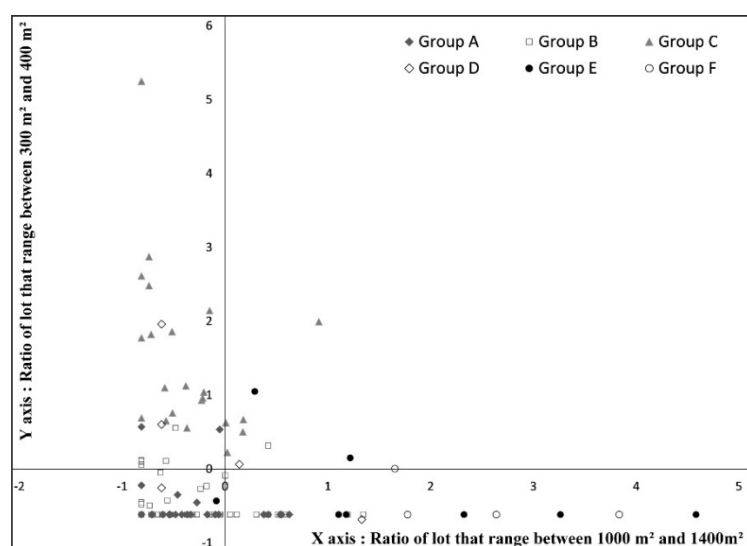
Figure 14. Scatter diagram (1).
