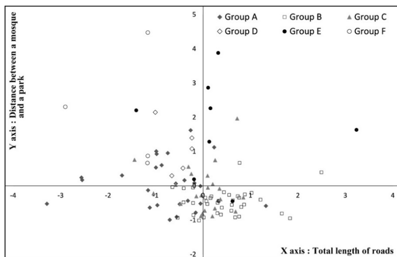
Figure 16. Scatter diagram (3).
