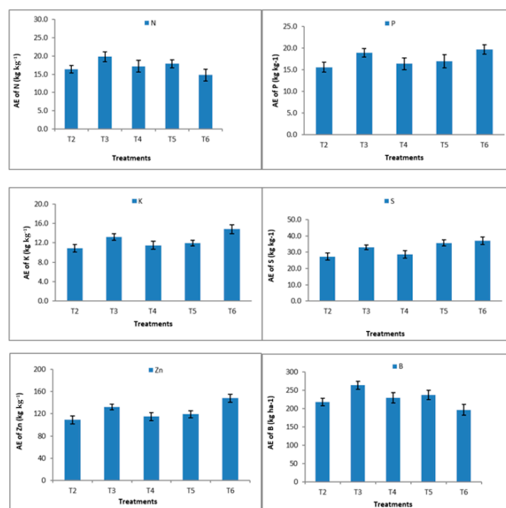
Figure 4. Effect of nutrient management practices on agronomic efficiency of N, P, K, S, Zn, and B in mungbean under the Aus–Aman–Lentil–Mungbean cropping system. T 2 =
