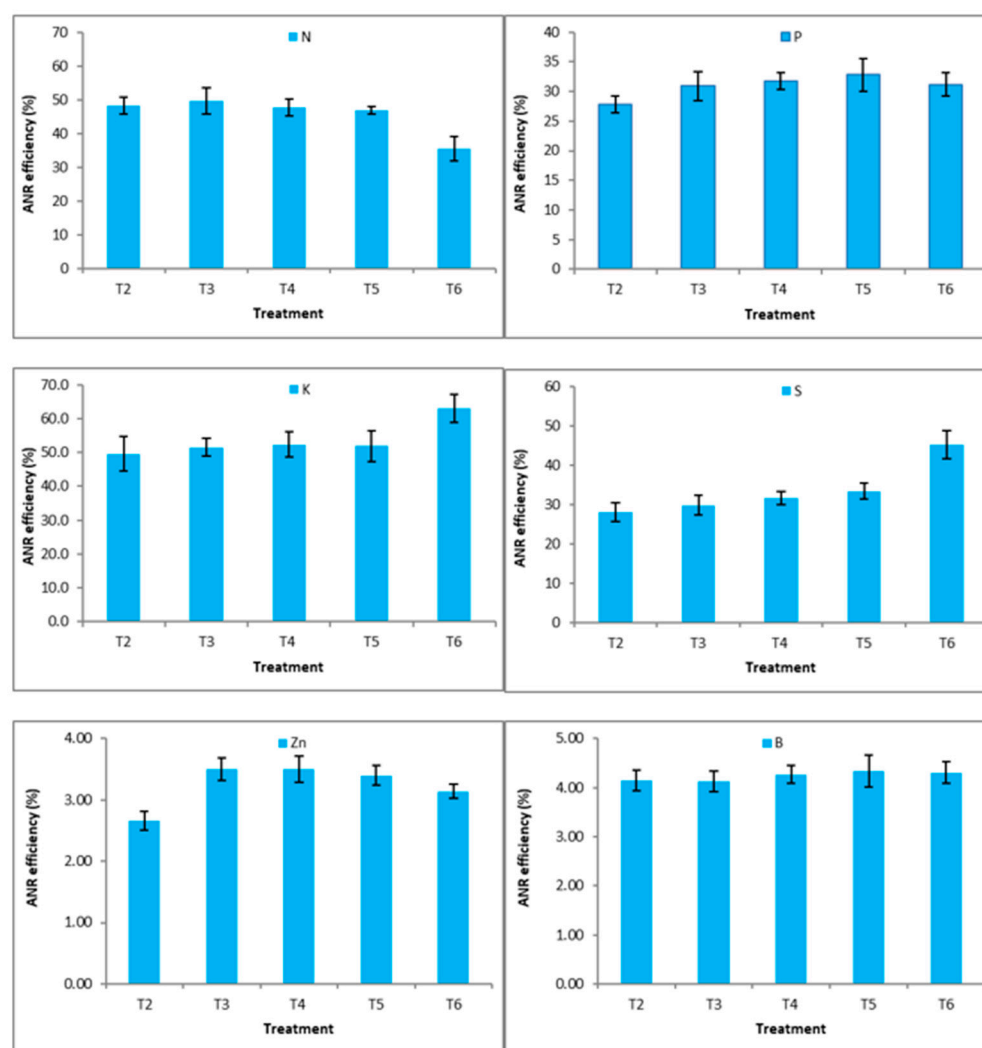
Figure 6. Effect of nutrient management practices on apparent N, P, K, S, Zn, and B recovery efficiency by the Aus–Aman–Lentil–Mungbean cropping system. T 2 = 50% recommended dose of
