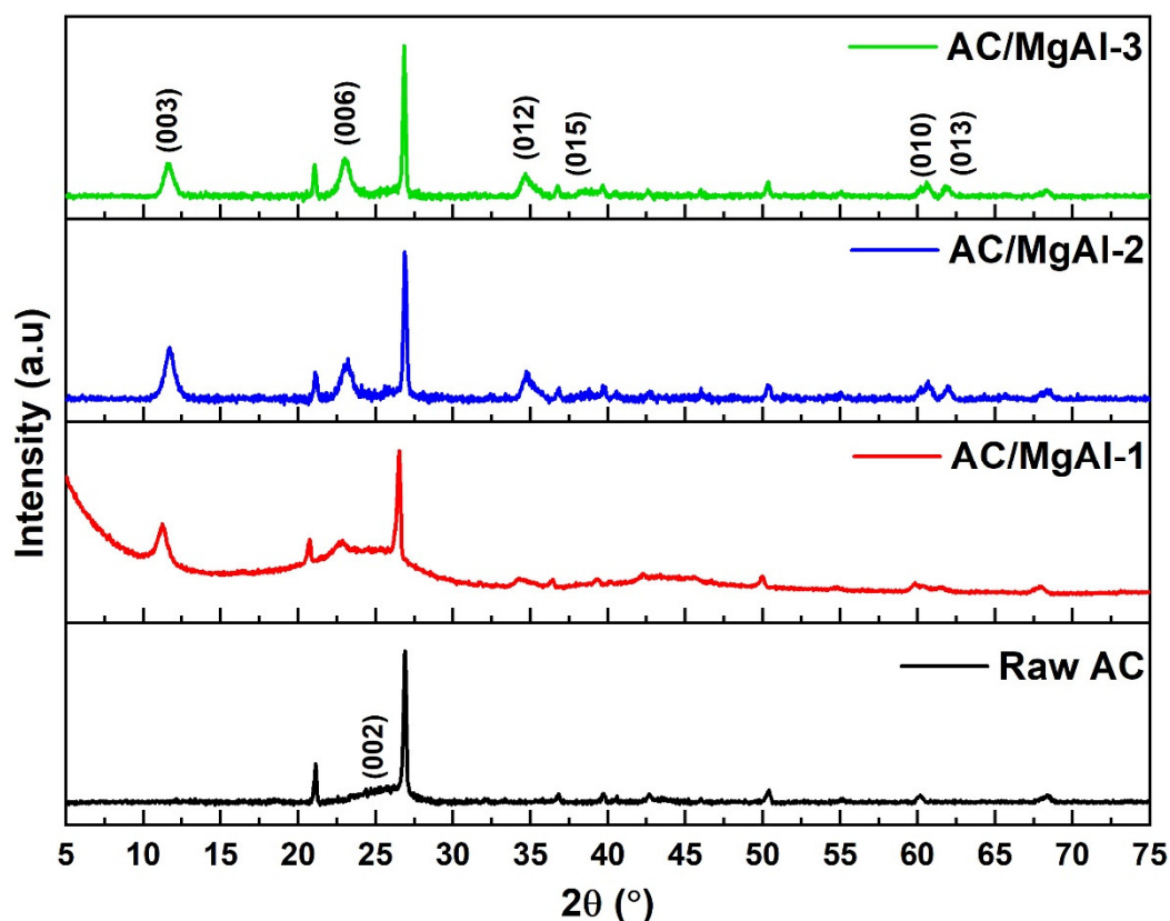
Figure 4. XRD patterns of AC/MgAl LDH composites.
