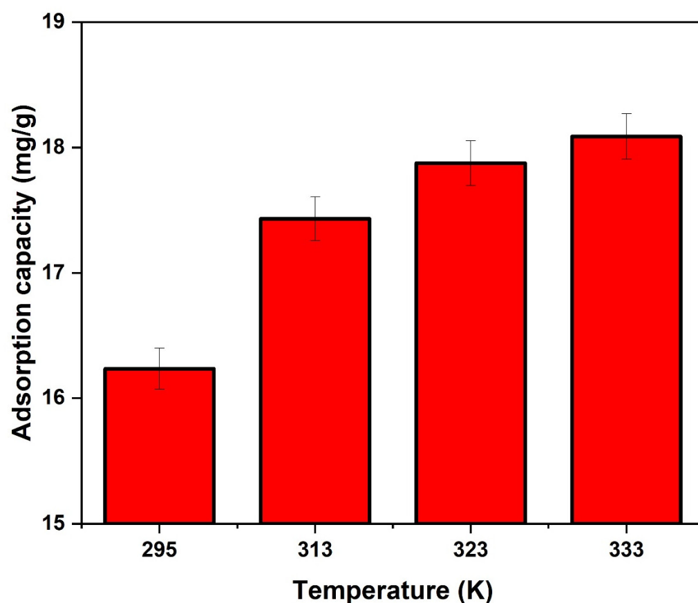
Figure 13. Effect of temperature on phosphate adsorption using AC/MgAl-3.
