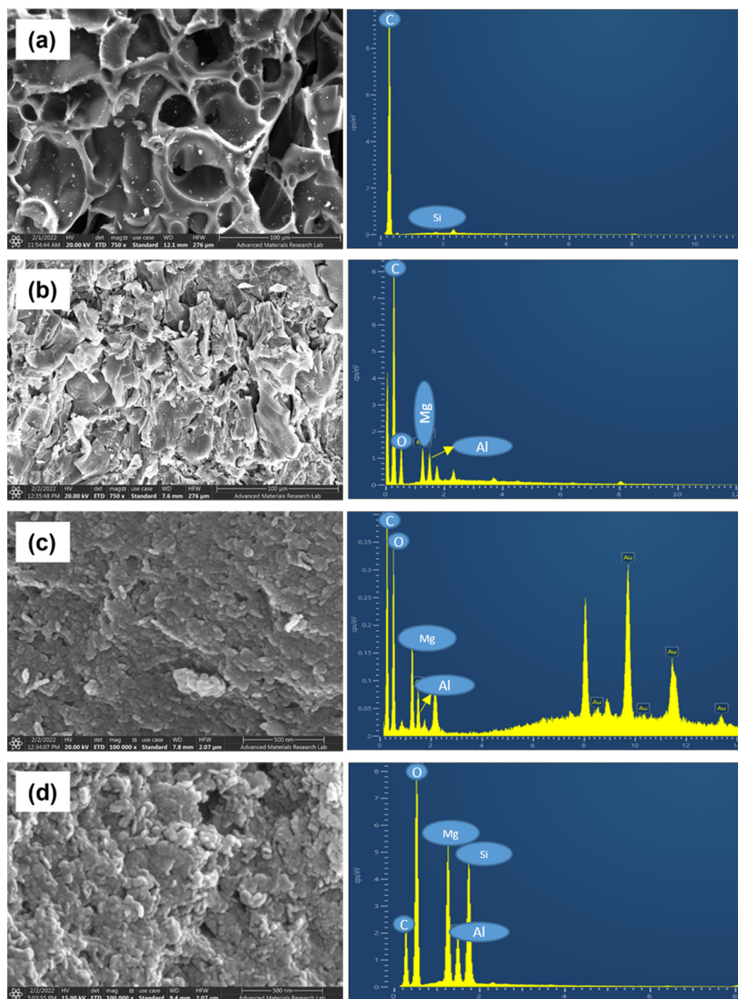
Figure 1. FE-SEM images of (a) raw AC, (b) AC/MgAl-1, (c) AC/MgAl-2, and (d) AC/MgAl-3 LDH composites.
