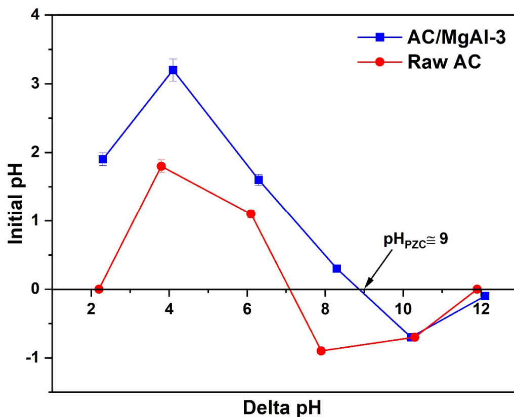
Figure 8. ZPC of raw AC and AC/MgAl-3 determined using the pH drift method.
