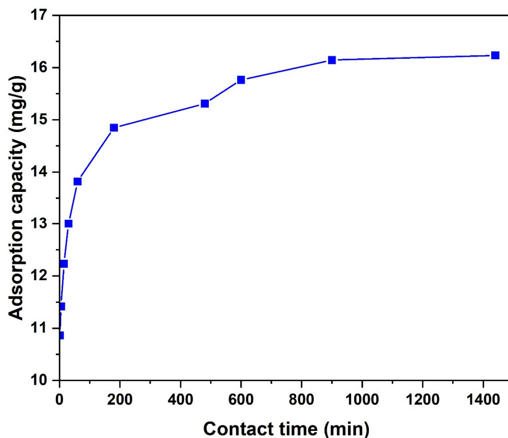
Figure 10. The relation between time and phosphate adsorption on AC/MgAl-3.
