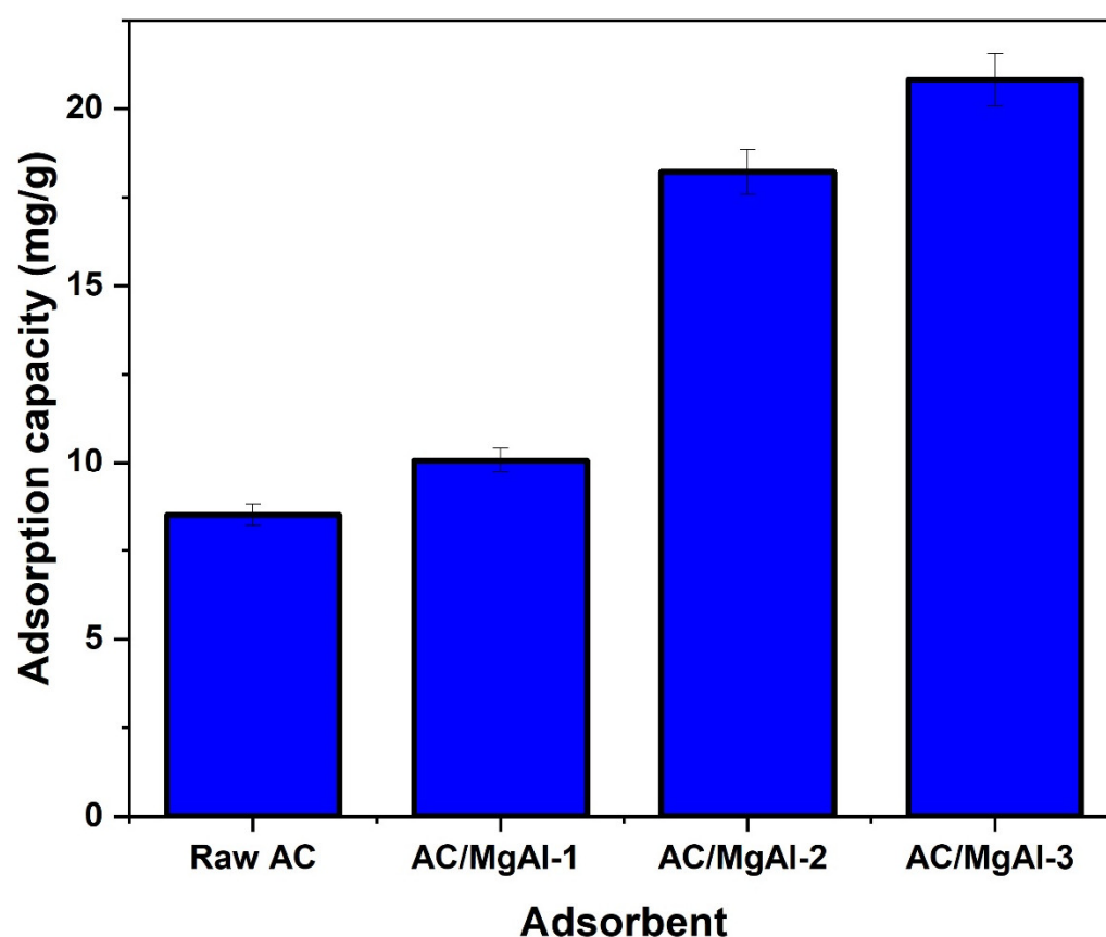
Figure 5. The effect of adsorbent type on phosphate adsorption capacity, pH = 6.3, C_0 = 50 mg/l, T = 22 °C.
