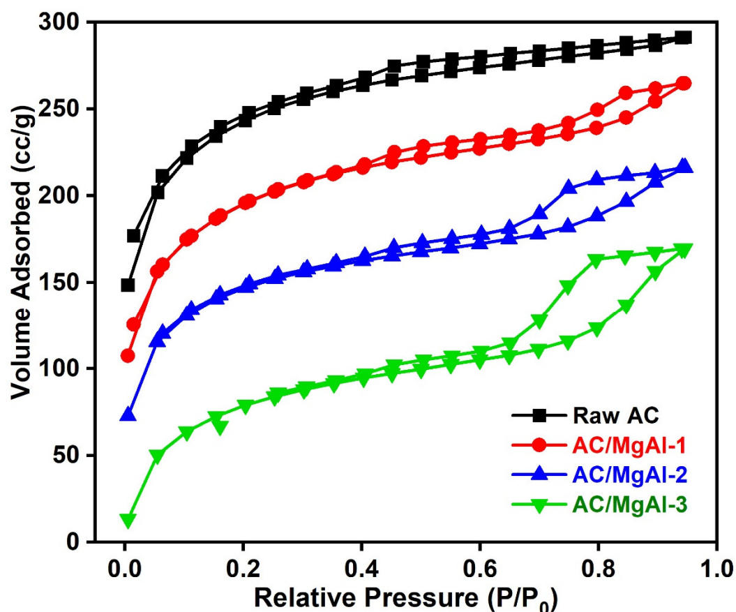
Figure 2. N 2 adsorption/desorption isotherms of AC/MgAl LDH composites.
