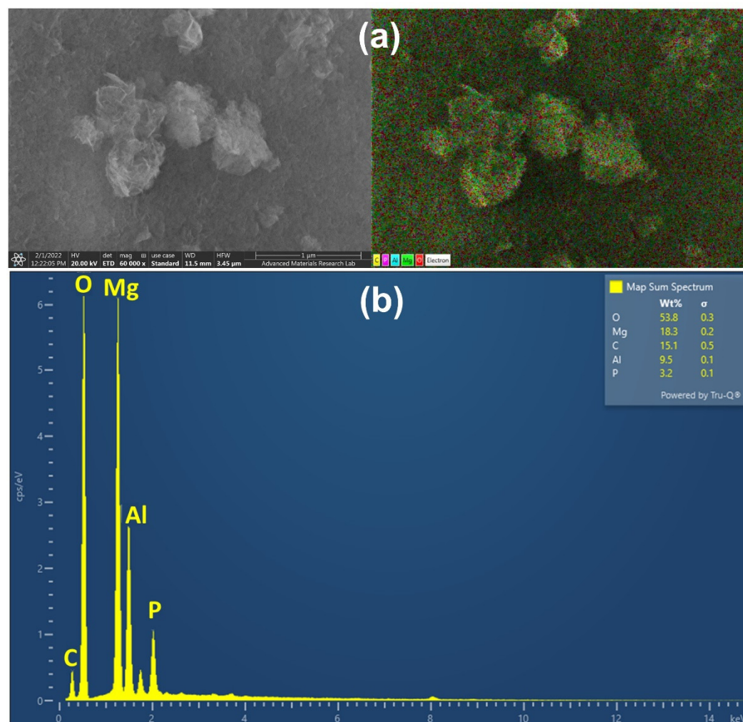
Figure 14. The (a) SEM, and (b) EDS analysis of AC/MgAl-3 LDH after phosphate adsorption.
