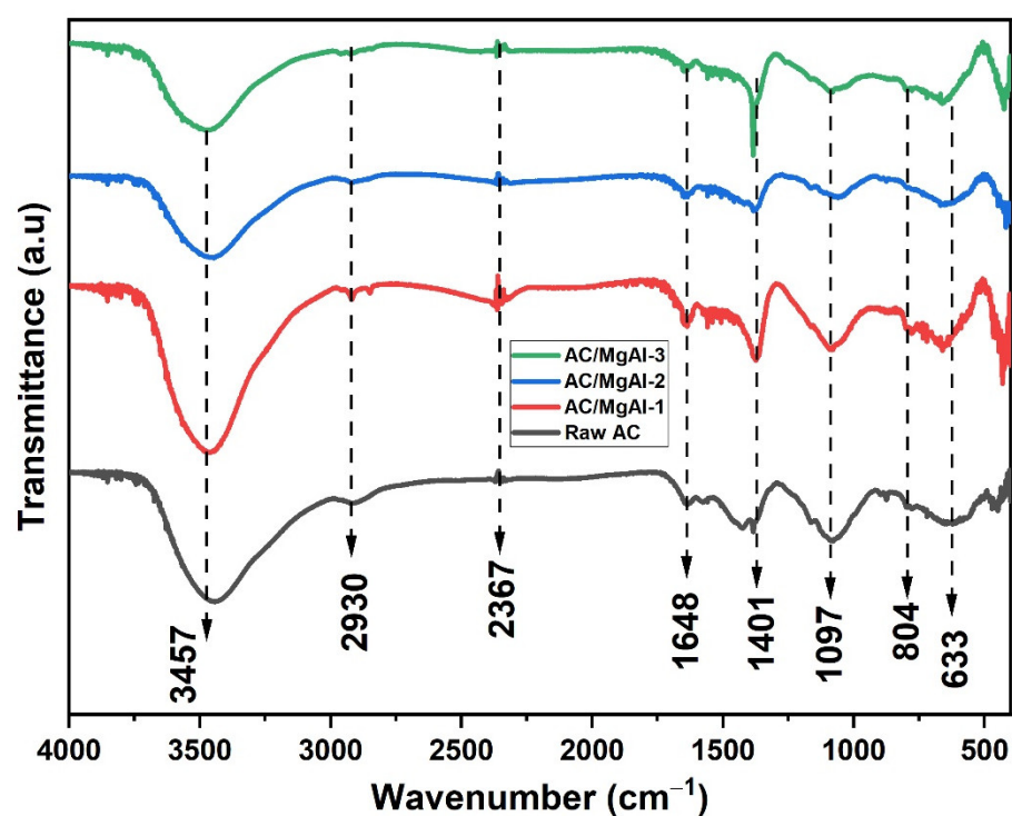
Figure 3. FT-IR spectra for AC/MgAl LDH composites.
