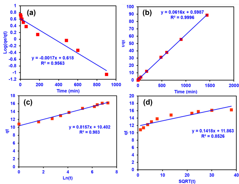
Figure 11. Kinetic models of phosphate adsorption on AC/MgAl-3 (a) the pseudo-first-order model, (b) the pseudo-second-order model, (c) the Elovich model, (d) the intraparticle diffusion model.
