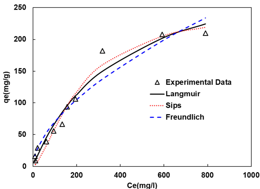
Figure 9. Nonlinear isotherms fitting of phosphate removal by AC/MgAl-3.
