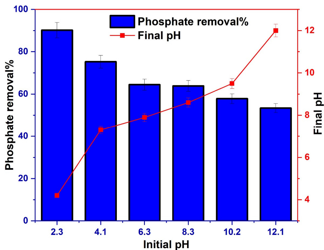
Figure 7. Effect of initial pH on the removal efficiency of phosphate and final pH.
