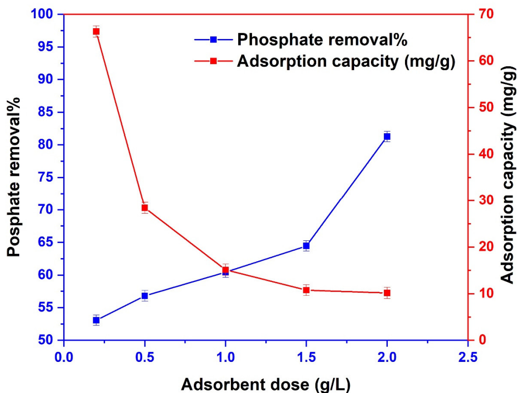
Figure 6. The effect of AC/MgAl-3 dosage on the removal efficiency and adsorption capacity of phosphate.
