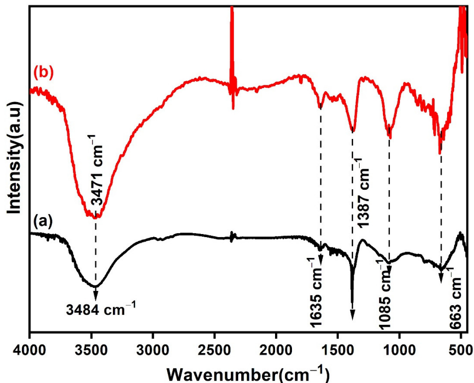
Figure 15. FT-IR spectra of AC/MgAl-3 before (a), and after (b) phosphate adsorption.
