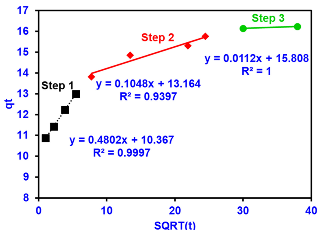
Figure 12. Three-steps intraparticle diffusion for phosphate removal on AC/MgAl-3.
