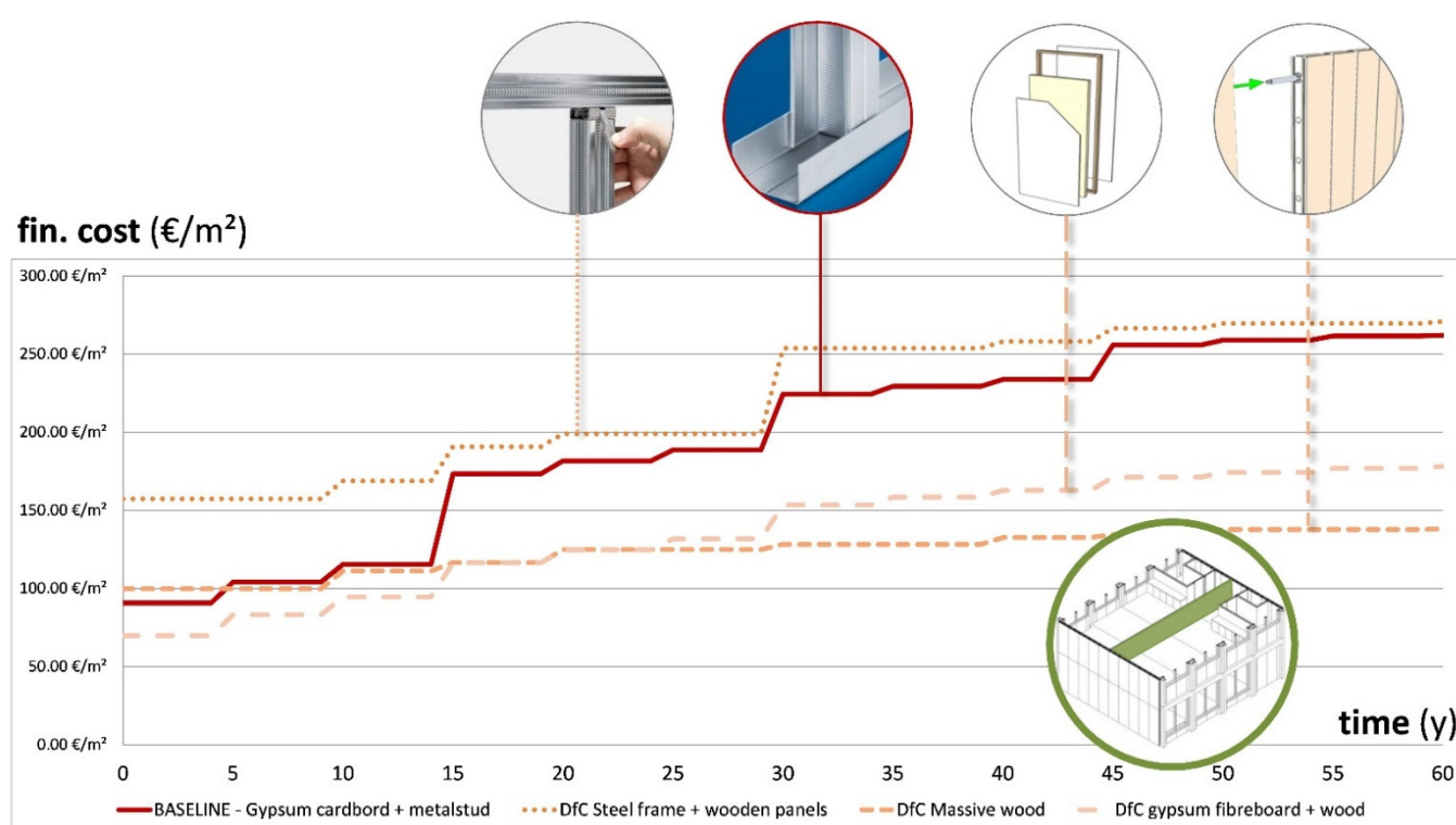
Figure 11. Financial cost per m 2 of Scenario 3, the dwelling-dividing interior wall. The baseline gypsum cardboard with metal stud solution is compared with the Design for Change (DfC) solutions steel frame with wooden panels, massive wood and gypsum fiberboard with wood. Transformation occurs every 15 years.
