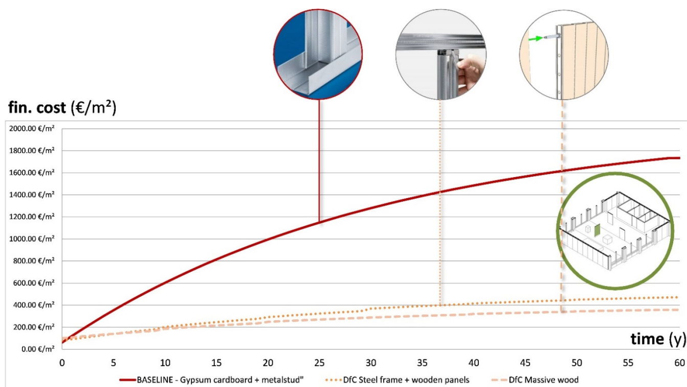
Figure 9. Financial cost per m 2 of Scenario 1, the quickly changing interior wall. The baseline gypsum cardboard with metal stud solution is compared with the Design for Change (DfC) solutions steel frame with wooden panels and massive wood. Transformation occurs every year in this scenario.
