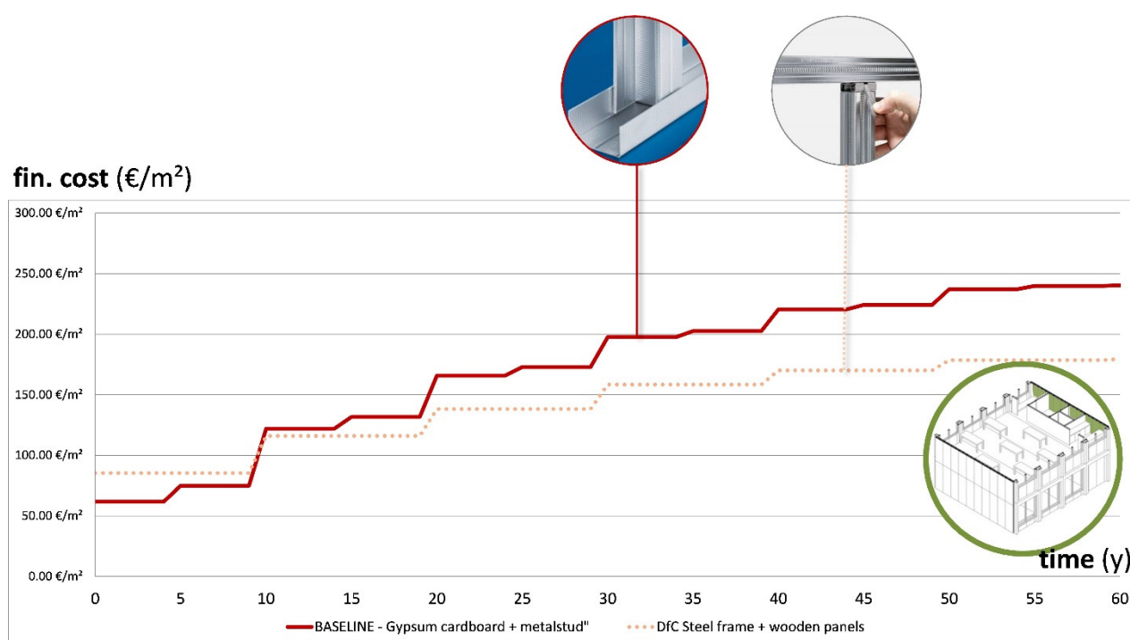
Figure 10. Financial cost per m 2 of Scenario 2, the technical interior wall. The baseline gypsum cardboard with metal stud solution is compared with the Design for Change (DfC) solution steel frame with wooden panels. Transformation occurs every 10 years.
