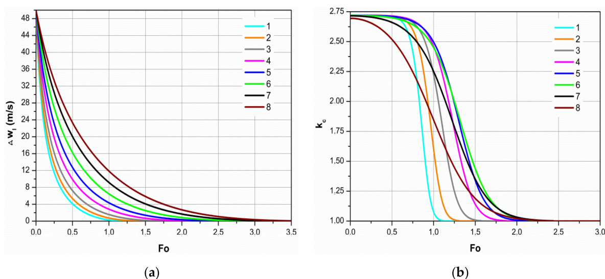
Figure 6. The dynamics of (a) the droplet slip in the gas flow and (b) the effective parameter of heat conductivity. The indications of the legend as in Figure 1.
