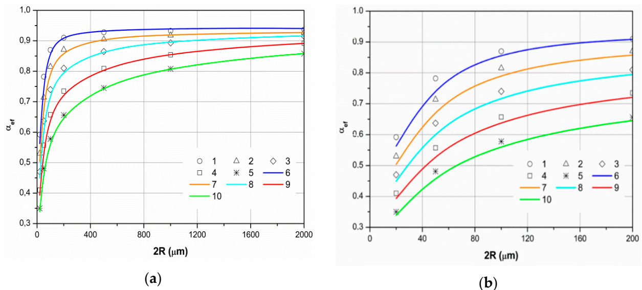
Figure 8. The water droplet effective absorptance ( \alpha_{ef} ): (a) in a wide range of droplet dispersity; (b) in small and medium-sized droplets. The points represent the results obtained during the numerical modeling of the volumetric absorption of spectral radiation based on the Mi theory [35]. The lines represent the results of the numerical modeling performed in this investigation of the volumetric absorption of spectral radiation in droplets based on the geometrical optics theory. The temperature of an external radiation source t_{sr} , °C: (1, 6) 377, (2, 7) 577, (3, 8) 777, (4, 9) 977; (5, 10) 1177; t_l = 100 °C.
