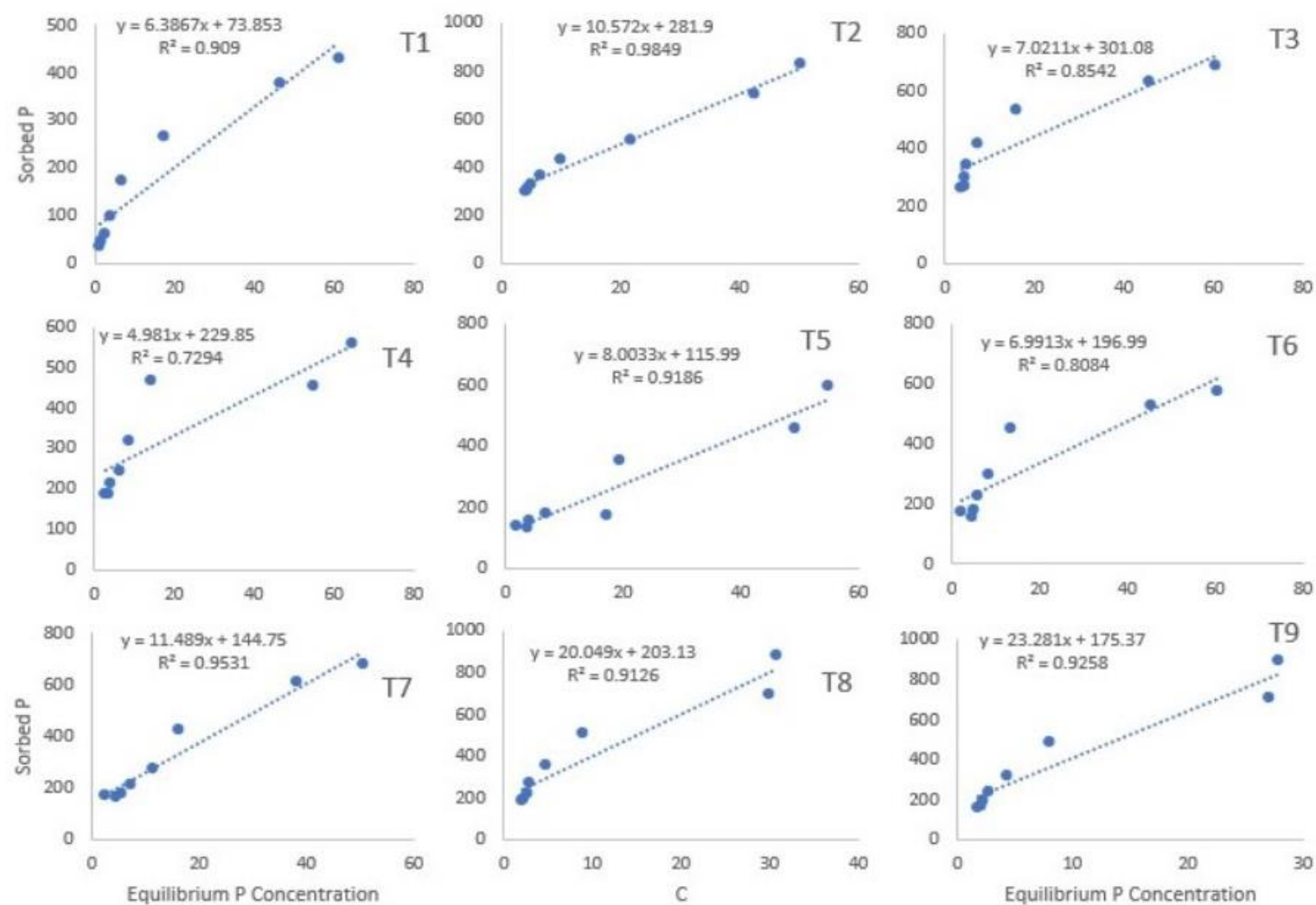
Figure S2. Sorption equation fitted using Langmuir (5 d incubation samples).
