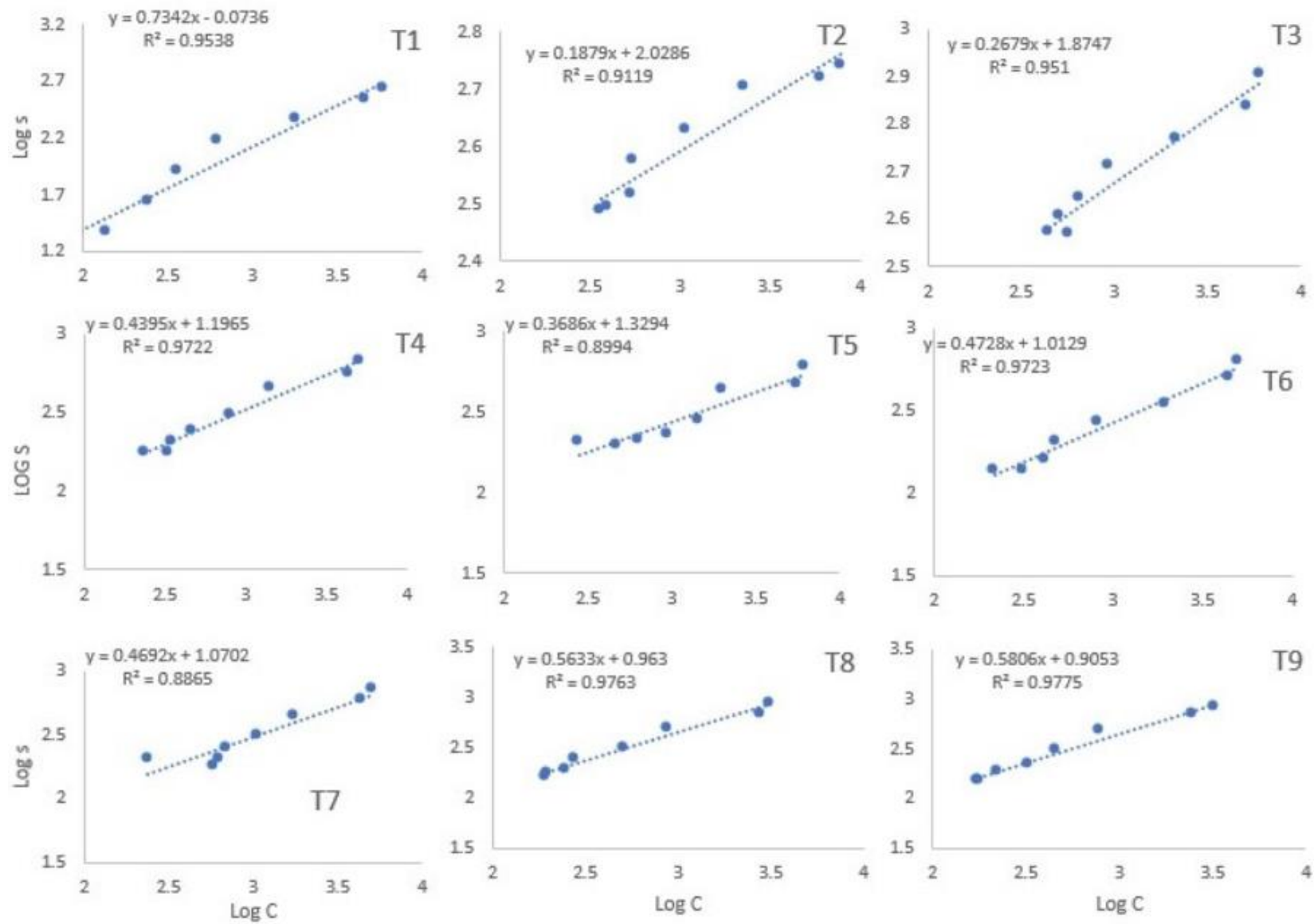
Figure S5. Sorption equation fitted using Freundlich (45 d incubation samples).
