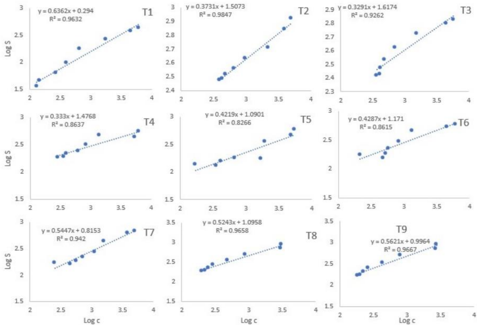
Figure S4. Sorption equation fitted using Freundlich (5 d incubation samples).
