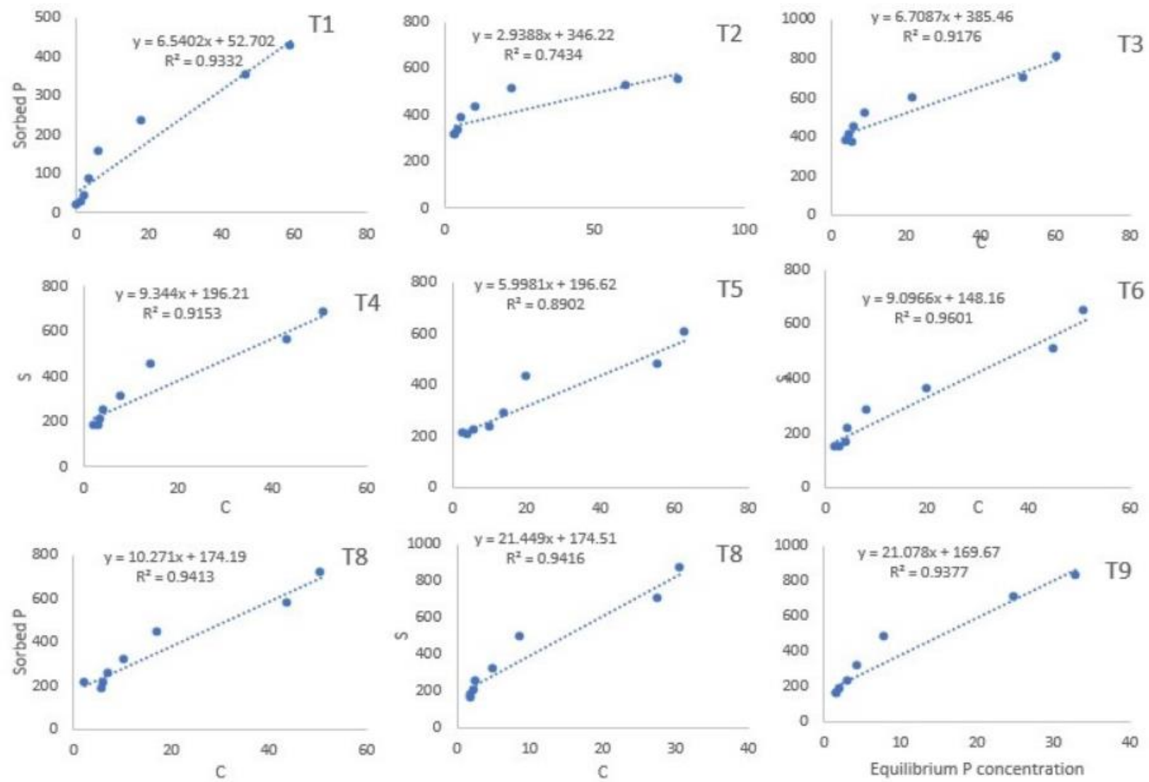
Figure S3. Sorption equation fitted using Langmuir (45 d incubation samples).
