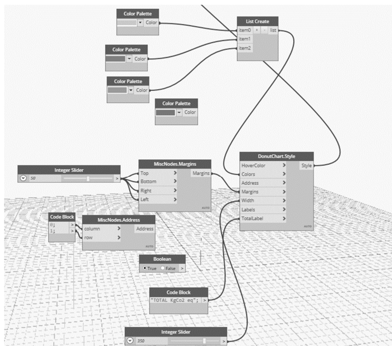
Figure 17. Choosing the chart style.
