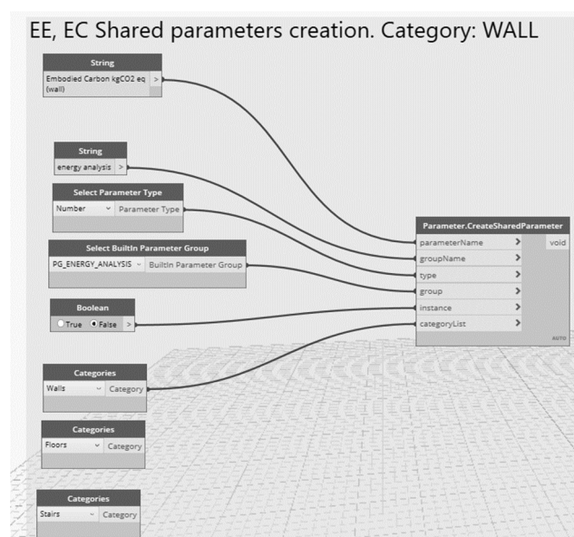
Figure 15. Script part related to Shared Parameters creation.
