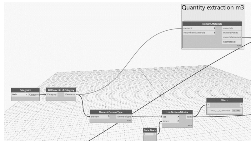
Figure 12. Quantities extraction from the Revit model.
