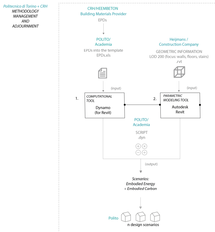
Figure 4. The methodological proposal.
