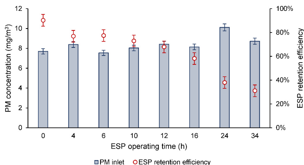
Figure 5. Evolution of ESP retention efficiency during operation.
