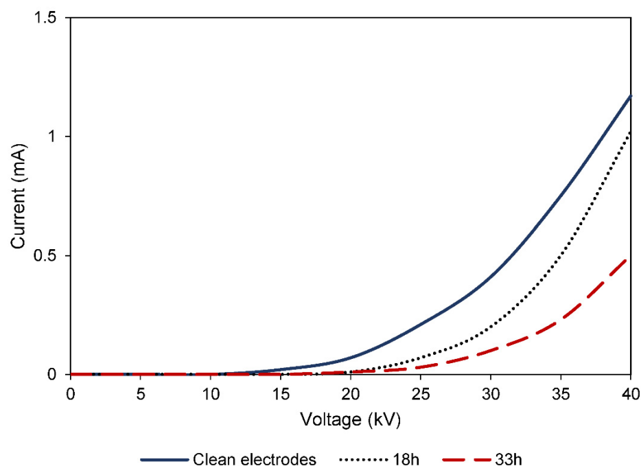
Figure 6. Evolution of the current–voltage curve during the operation of the ESP.
