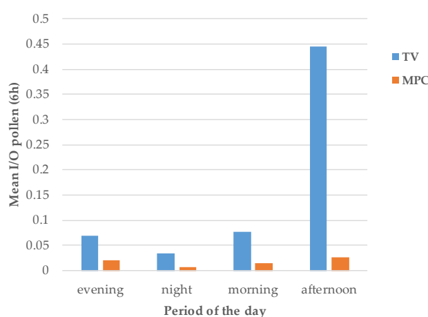
Figure 11. Mean I/O ratio (6-h average) during the daily time ranges (evening, night, morning and afternoon) in TV and MPC.
