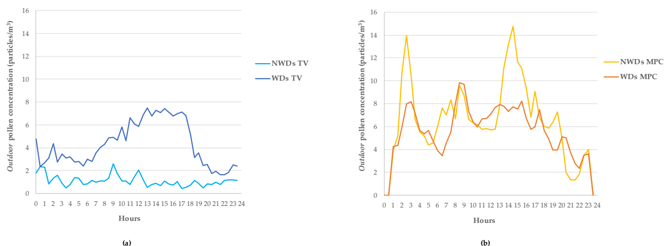
Figure 6. Daily trend of the outdoor pollen concentration for TV (a) and MPC (b) in NWDs and WDs.
