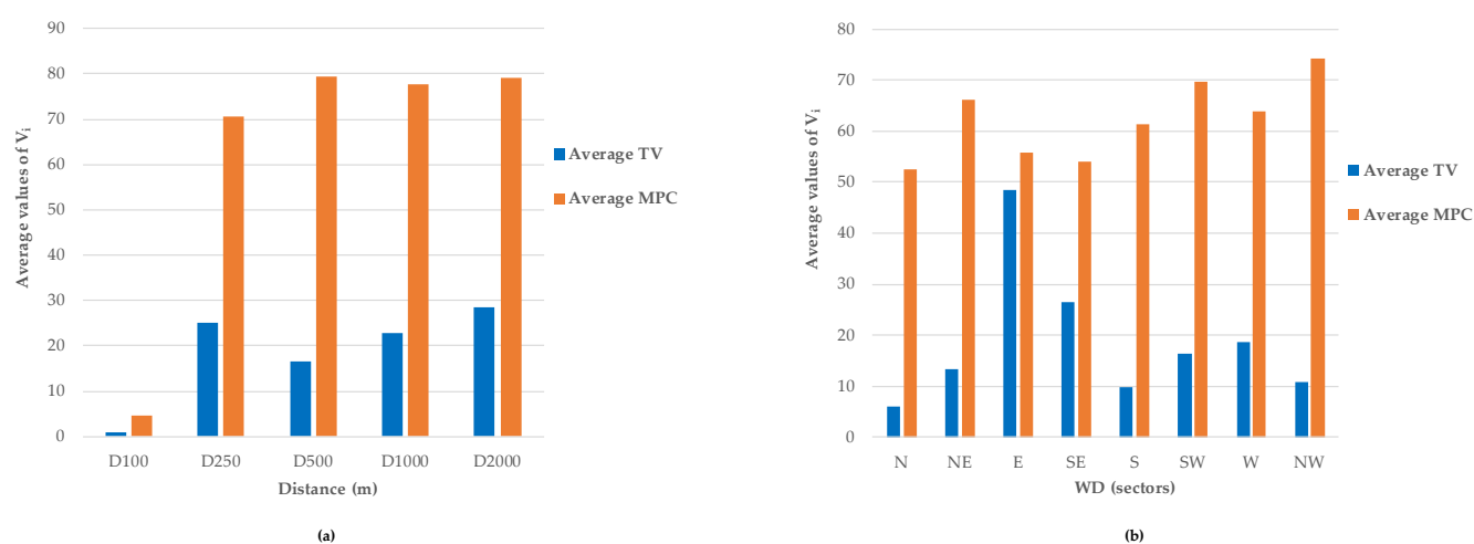
Figure 4. The average values of V_i as function of distance (a) and the wind direction (b), for TV and MPC.
