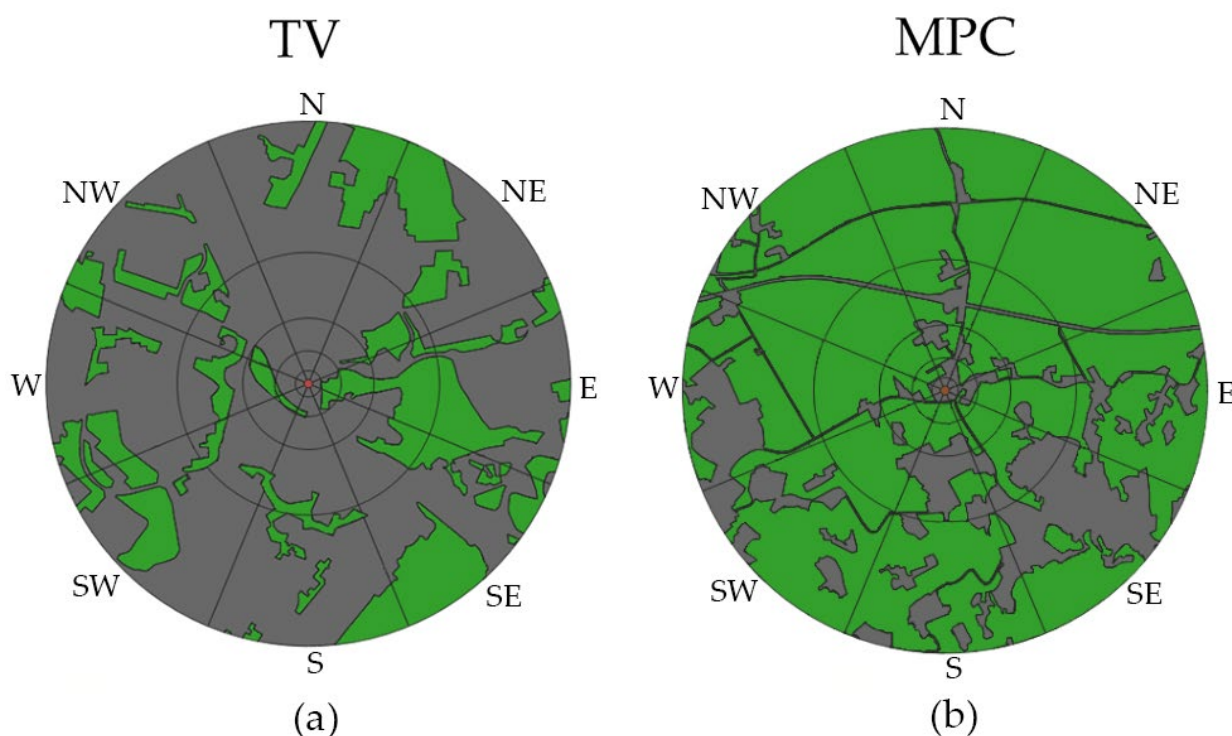
Figure 2. Maps of the artificial surfaces (in grey) and green areas (in green) present in a 2 km radius around the pollen samplers in TV (a) and MPC (b). In the maps, the concentric circumferences of 1 km, 0.5 km, 0.25 km and 0.1 km radius and the octants corresponding to cardinal directions are also shown.
