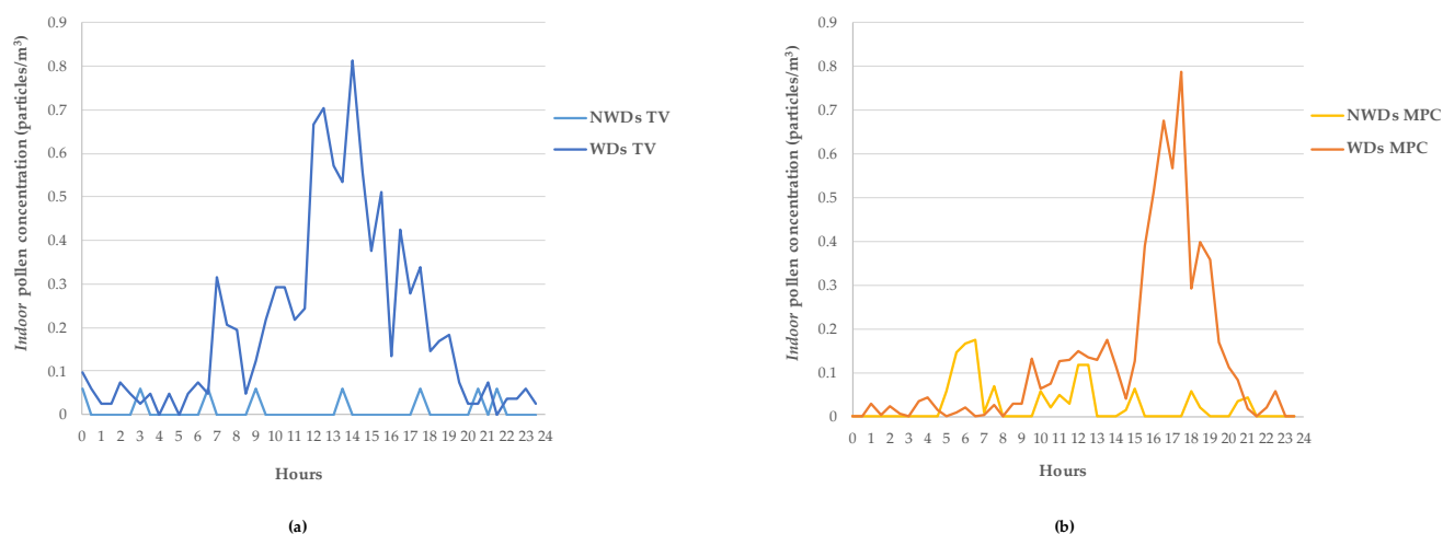
Figure 7. Daily trend of the indoor pollen concentration for TV (a) and MPC (b) in NWDs and WDs.
