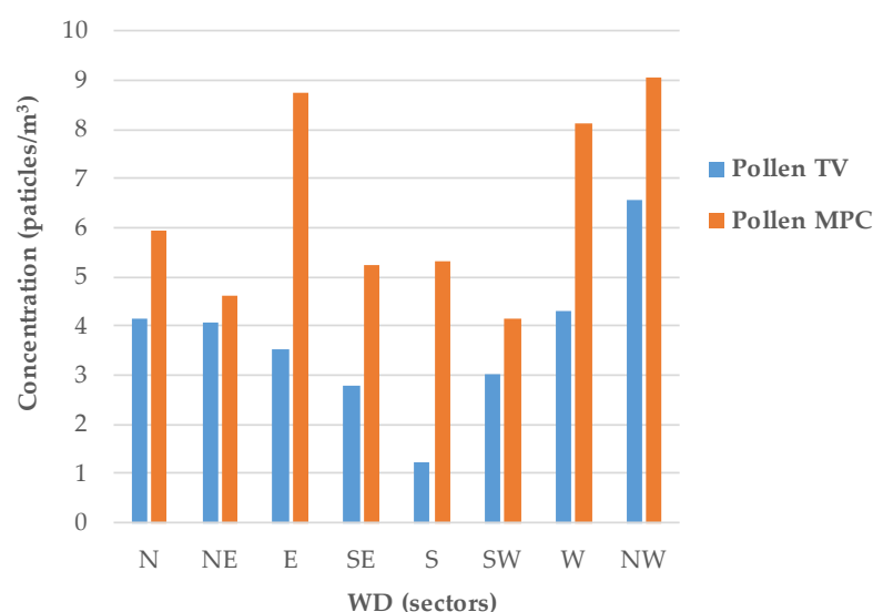
Figure 5. Pollen concentration at TV and MPC as function of measured wind direction.
