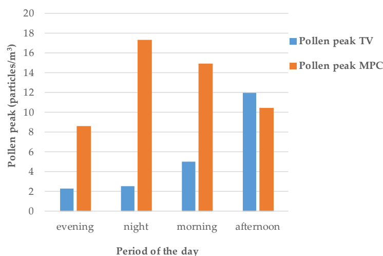
Figure 9. Mean pollen peak during the daily time ranges (evening, night, morning and afternoon) in TV and MPC.
