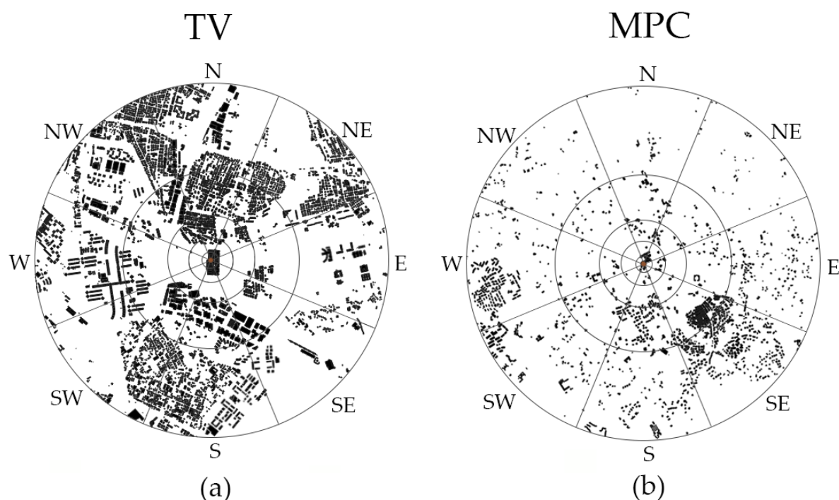
Figure 1. Maps of the buildings (in black) present in a 2 km radius around the pollen samplers in TV (a) and MPC (b). In the maps, the concentric circumferences of 1 km, 0.5 km, 0.25 km and 0.1 km radius and the octants corresponding to cardinal directions are also shown.
