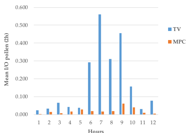
Figure 10. Daily evolution of the mean I/O ratio (two hours average) in TV and MPC.
