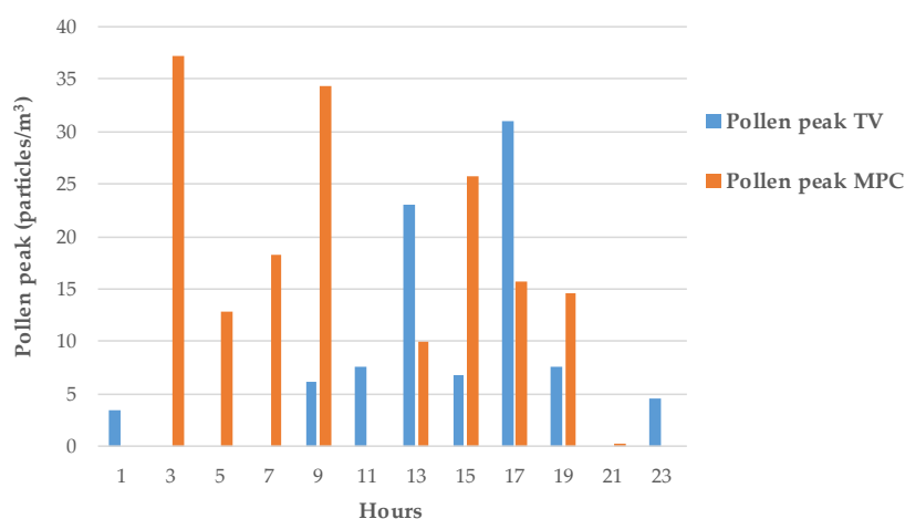
Figure 8. Mean pollen peak during the day in TV and MPC.
