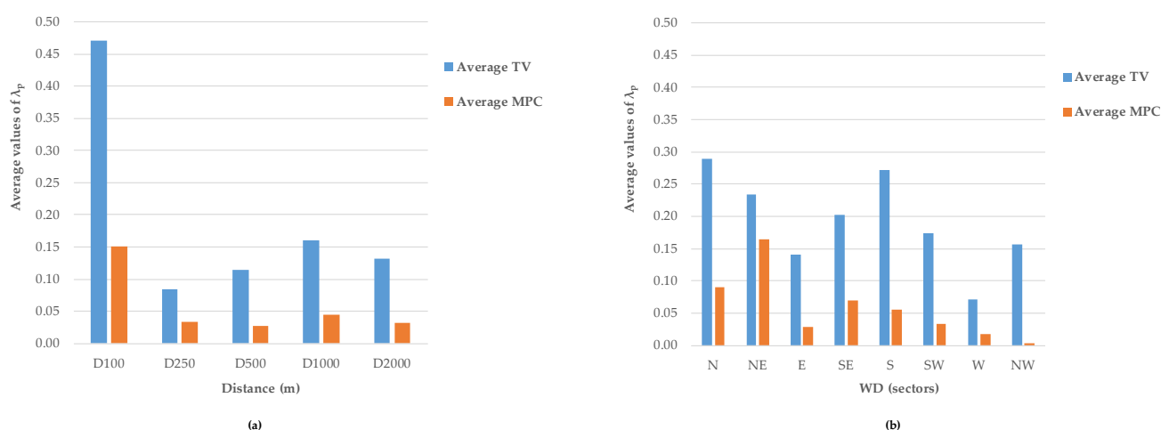
Figure 3. The average values of \lambda_p as function of the distance (a) and the wind direction (b), for TV and MPC.
