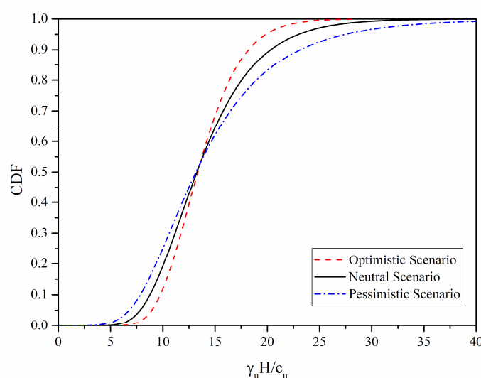
Figure 4. Curves of CDF under three probabilistic scenarios with the critical Scheme 5. 1.3. Influence on Sobol' Index.
