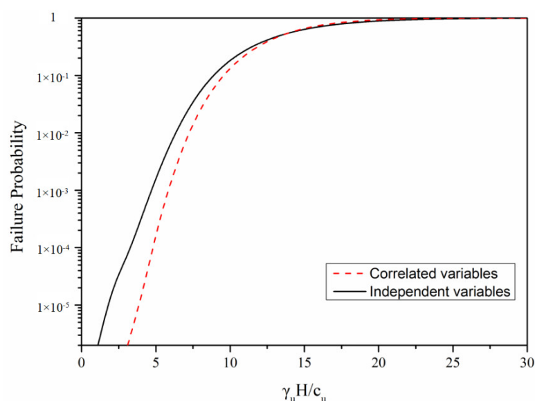
Figure 9. Impact of correlation on failure probability as a function of the critical slope height normalized by the soil unit weight and cohesion.
