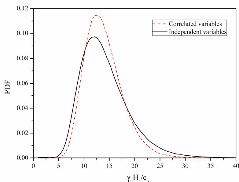
Figure 7. Impact of correlation on PDF with the critical slope height normalized by the soil unit weight and cohesion.
