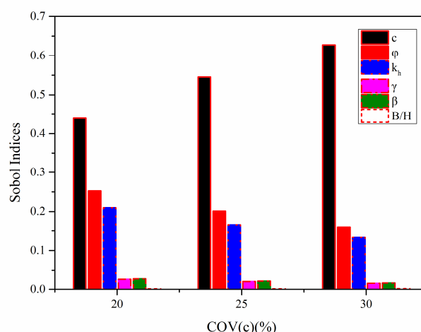
Figure 5. Impact of COVs on Sobol' Index for cohesion c .
