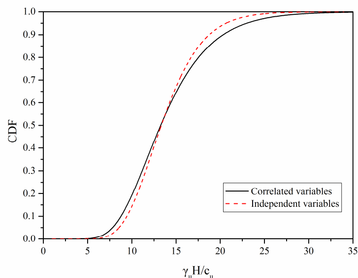
Figure 8. Impact of correlations on CDF with the critical slope height normalized by the soil unit weight and cohesion.
