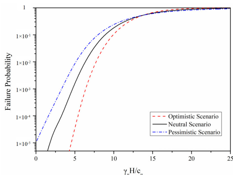
Figure 3. Failure probability under three uncertainty levels as a function of the critical slope height normalized by the soil unit weight and cohesion.
