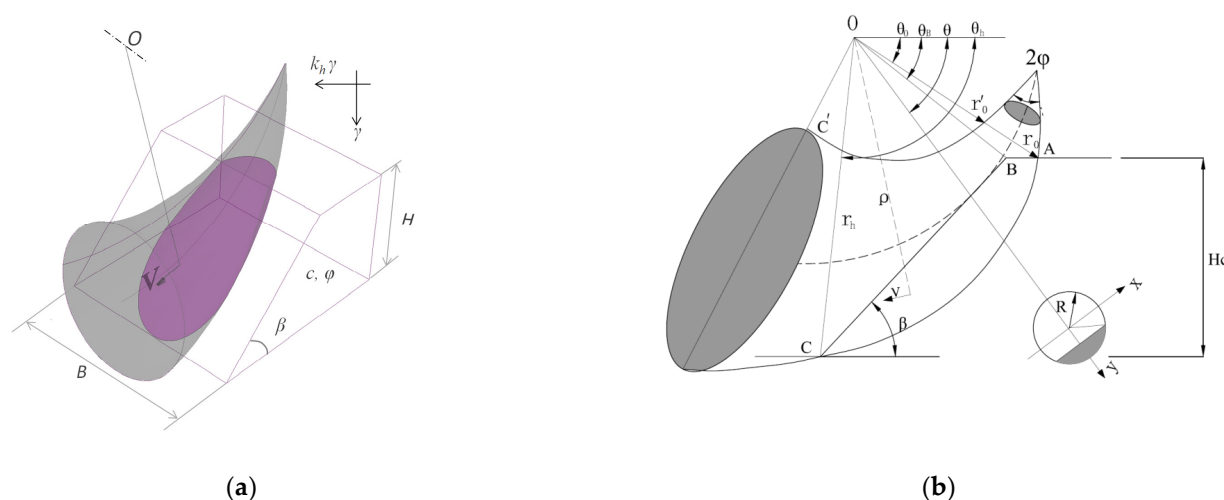
Figure 1. Sketch of (a) the slope problem under study and (b) the associated 3D rotational failure mechanism.
