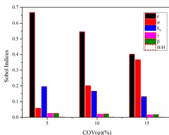
Figure 6. Impact of COVs on Sobol' Index for friction angle \varphi .
