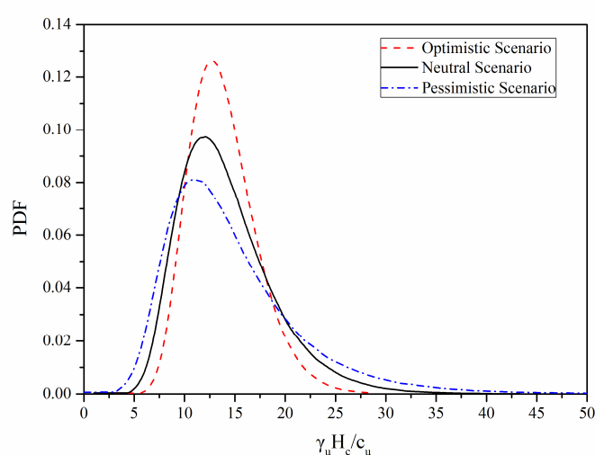
Figure 2. Impact of uncertainty level on PDF with the critical slope height normalized by the soil unit weight and cohesion.
