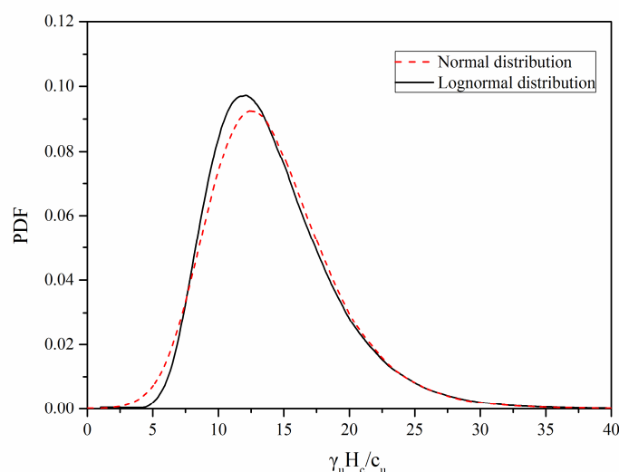
Figure 10. Impact of distribution types on PDF.
