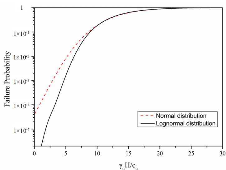
Figure 11. Impact of distribution types on failure probability.
