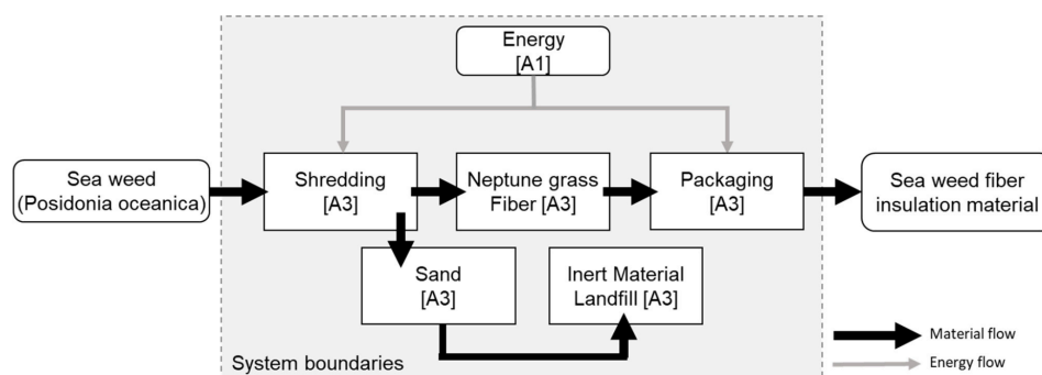
Figure 3. Production system of the insulation material made from seaweed; striped lining marks the considered system boundaries.
