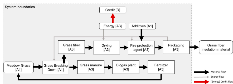
Figure 2. Production system of the insulation material made from meadow grass.
