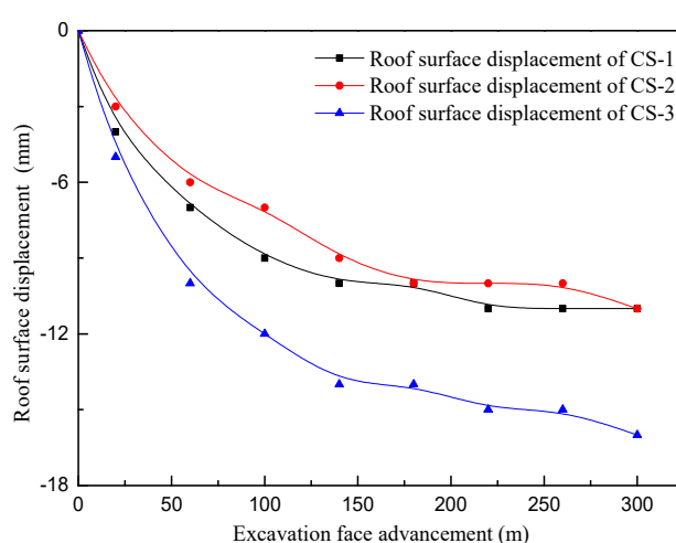
Figure 10 Relationship between roof surface displacement and excavation face advancement.
