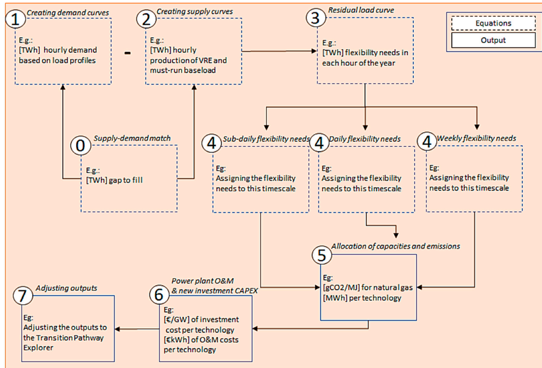
Figure 11. Calculation logic of the storage requirements module.
