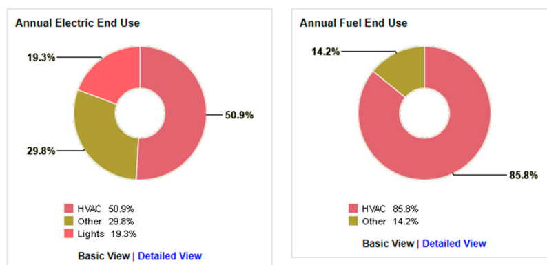
Figure 12. Annual electric and fuel end-use for HVAC, lights, and other (miscellaneous equipment) in the eastern single facade. © By author.
