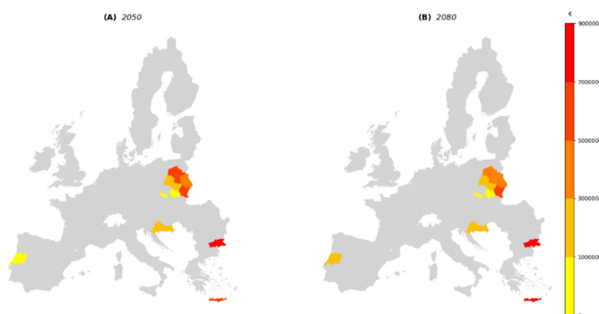
Figure 6. The total value of unaffordability under the PPP-insurance market, in Euros (2013), for the selected regions where a tipping-point is expected.
