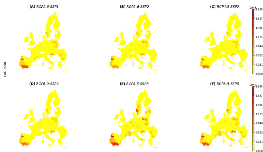
Figure A4. Expected annual damage in 2050 under RCP2.6-SSP1 (panel A); RCP2.6-SSP2 (panel B); RCP4.5-SSP2 (panel C); RCP6.0-SSP2 (panel D); RCP8.5-SSP3 (panel E); RCP8.5-SSP5 (panel F).
