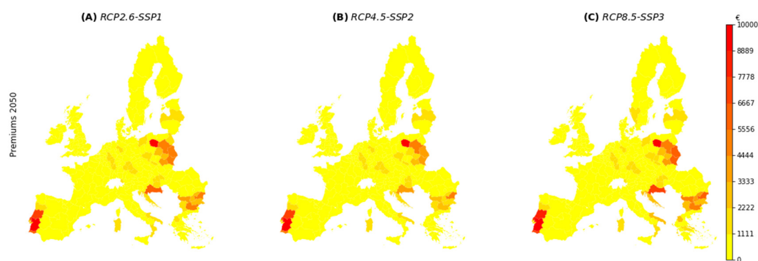
Figure A7. Flood insurance premiums in 2050 on NUTS2-level, under current national insurance systems, shown for RCP2.6-SSP1 (panel A); RCP4.5-SSP2 (panel B); RCP8.5-SSP3 (panel C).
