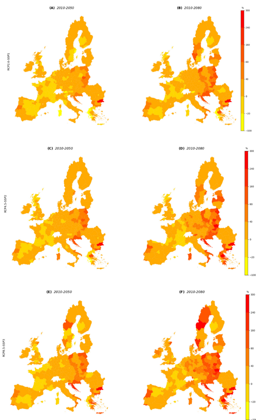
Figure 2. The percentage change of unaffordability under status-quo insurance arrangements for households in high-risk areas under the RCP2.6-SSP1 (panels A and B), RCP4.5-SSP2 (panels C and
