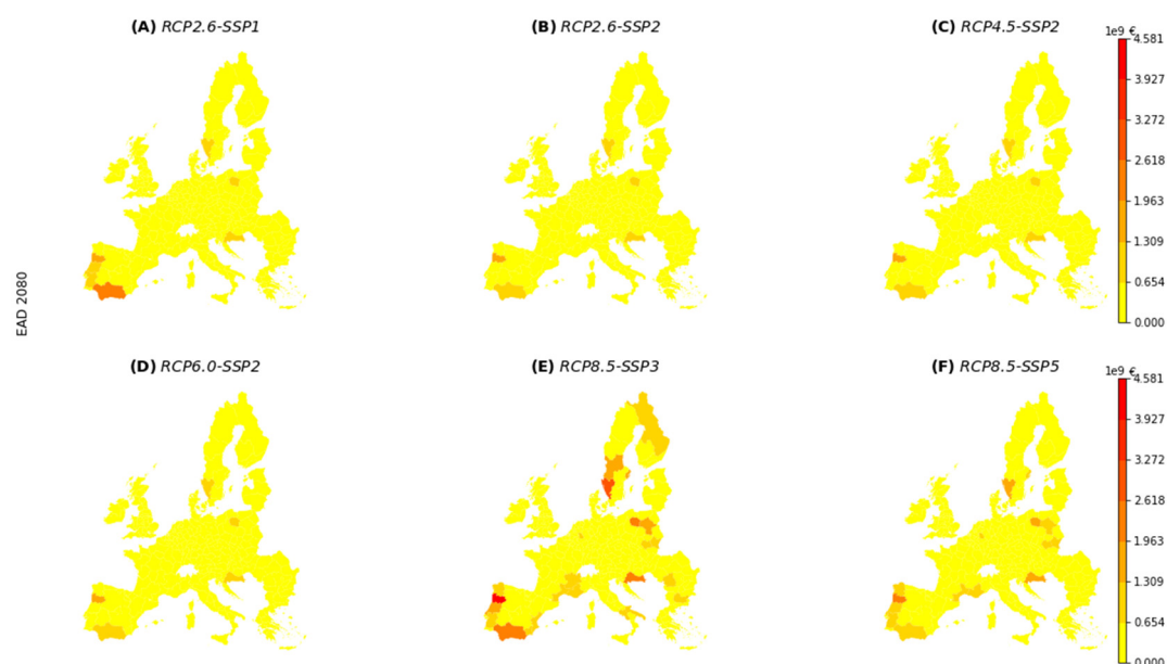
Figure A5. Expected annual damage in 2080 under RCP2.6-SSP1 (panel A); RCP2.6-SSP2 (panel B); RCP4.5-SSP2 (panel C); RCP6.0-SSP2 (panel D); RCP8.5-SSP3 (panel E); RCP8.5-SSP5 (panel F).
