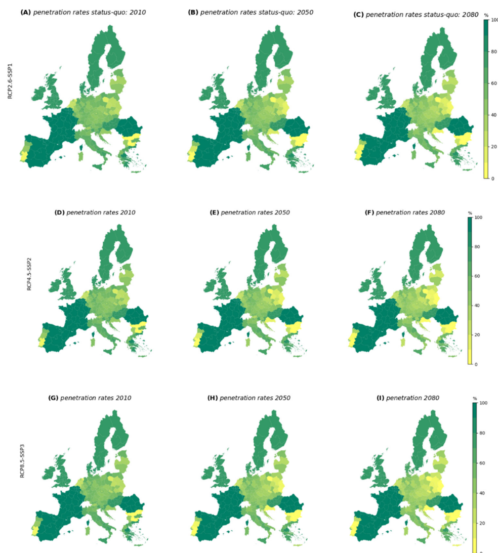
Figure 3. Flood insurance penetration rates under status-quo insurance arrangements for households in high-risk areas under the RCP2.6-SSP1 (Figure 3 A–C), RCP4.5-SSP2 (Figure 3 D–F), and RCP8.5-SSP3 (Figure 3 G–I) scenarios of climate and socio-economic change for the periods 2010 (left), 2050 (middle), and 2080 (right).
