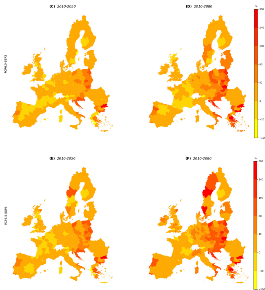
Figure A1. The percentage change of unaffordability under status-quo insurance arrangements for households in high-risk areas under the RCP2.6-SSP2 (panels A and B), RCP6.0-SSP2 (panels C and D), and RCP8.5-SSP5 (panels E and F) scenarios of climate and socio-economic change for the periods 2010–2050 (left) and 2010–2080 (right). Unaffordability is measured as the percentage of the population in high-risk areas that cannot afford the insurance premium.
