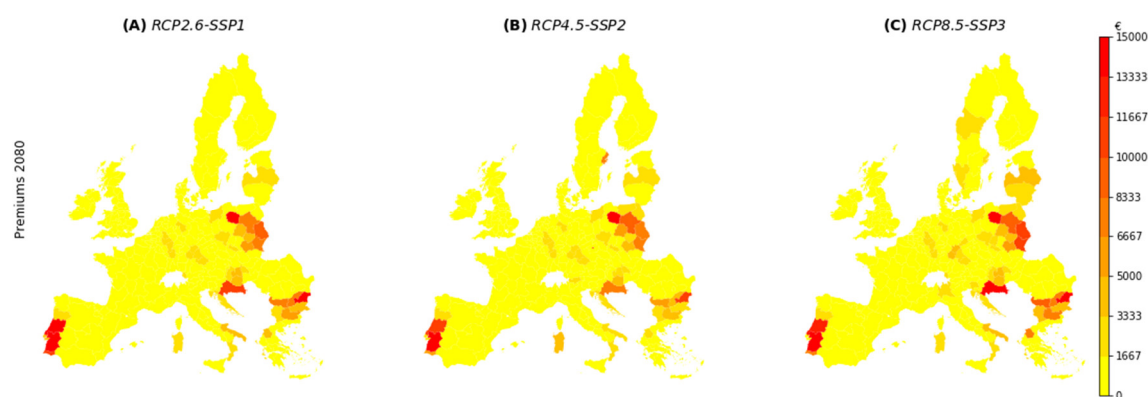
Figure A8. Flood insurance premiums in 2080 on NUTS2-level, under current national insurance systems, shown for RCP2.6-SSP1 (panel A); RCP4.5-SSP2 (panel B); RCP8.5-SSP3 (panel C).
