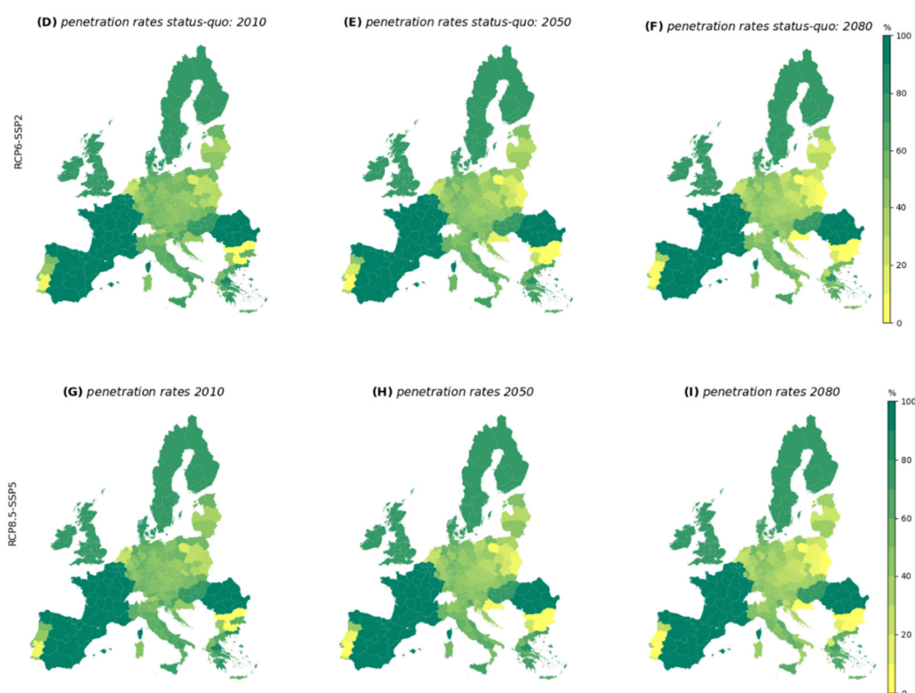
Figure A2. Flood insurance penetration rates under status-quo insurance arrangements for households in high-risk areas under the RCP2.6-SSP2 (panels A–C), RCP6.0-SSP2 (panels D–F), and RCP8.5-SSP5 (panels G–I) scenarios of climate and socio-economic change for the periods 2010 (left), 2050 (middle), and 2080 (right).
