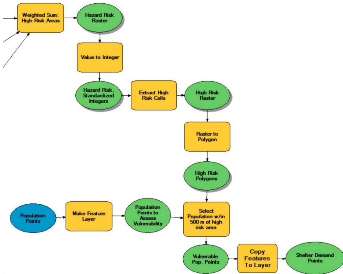
Figure S1. Automated AHP. (a) Model Builder tool; (b) Corresponding hierarchy components; (c) Detail of Model Builder section A; (d) Detail of Model Builder section B; (e) Detail of Model Builder section C; (f) Detail of Model Builder section D.
