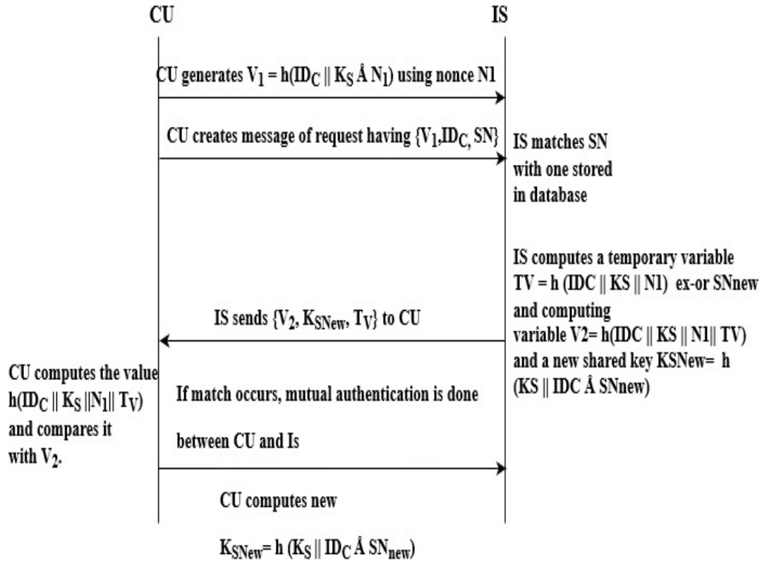
Figure 6. Authentication process of HLSF.
