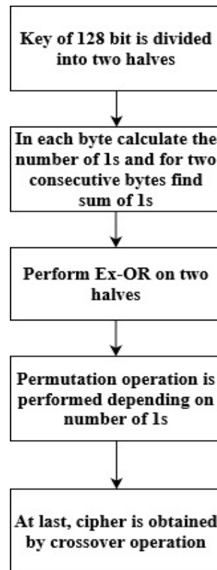
Figure 7. Data security process of HLSF.
