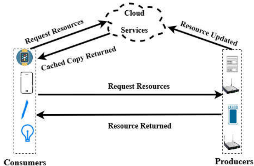
Figure 3. Object security framework for IoT (OSCAR) framework.
