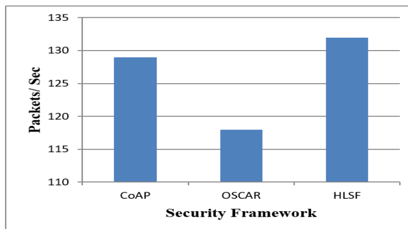
Figure 11. Communication Rate for CoAP, OSCAR, and HLSF.
