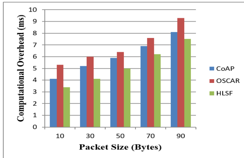
Figure 10. Computational overhead for CoAP, OSCAR, and HLSF.
