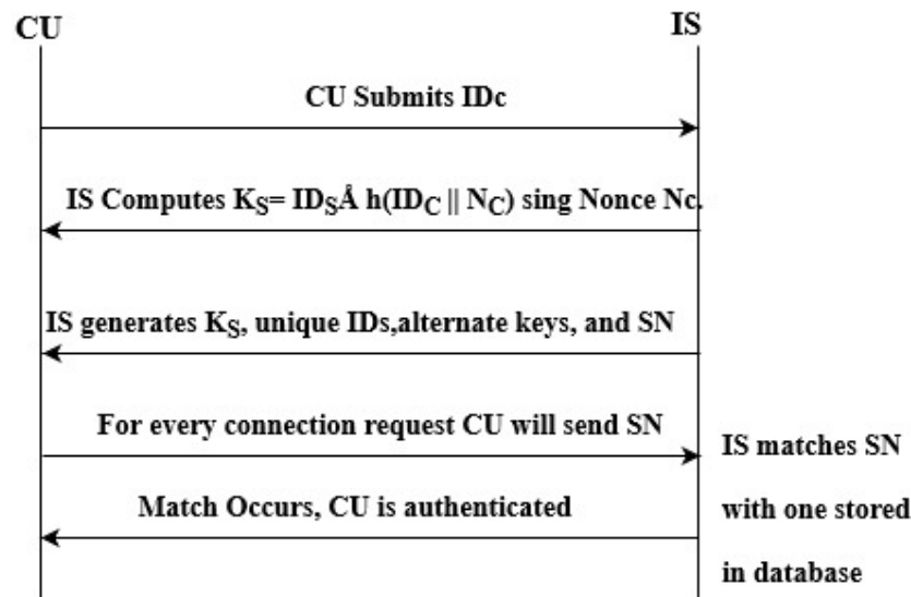
Figure 5. Registration process of HLSF.
