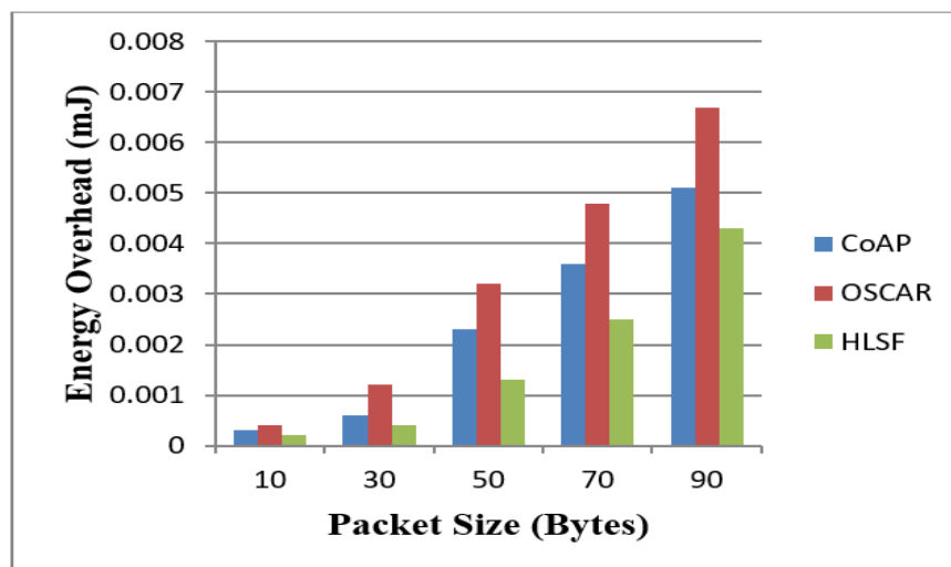
Figure 9. Energy overhead for CoAP, OSCAR, and HLSF.
