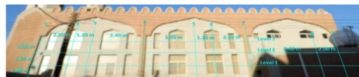
Outdoor Western Elevation for Noor El-Eeman Mosque
