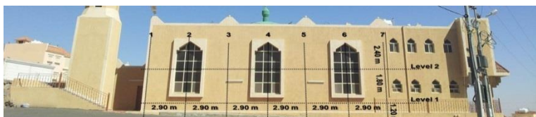
Outdoor Western Elevation for Al-Hayyani Mosque
