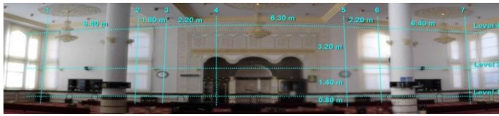
Indoor North Elevation for Noor El-Eeman Mosque
