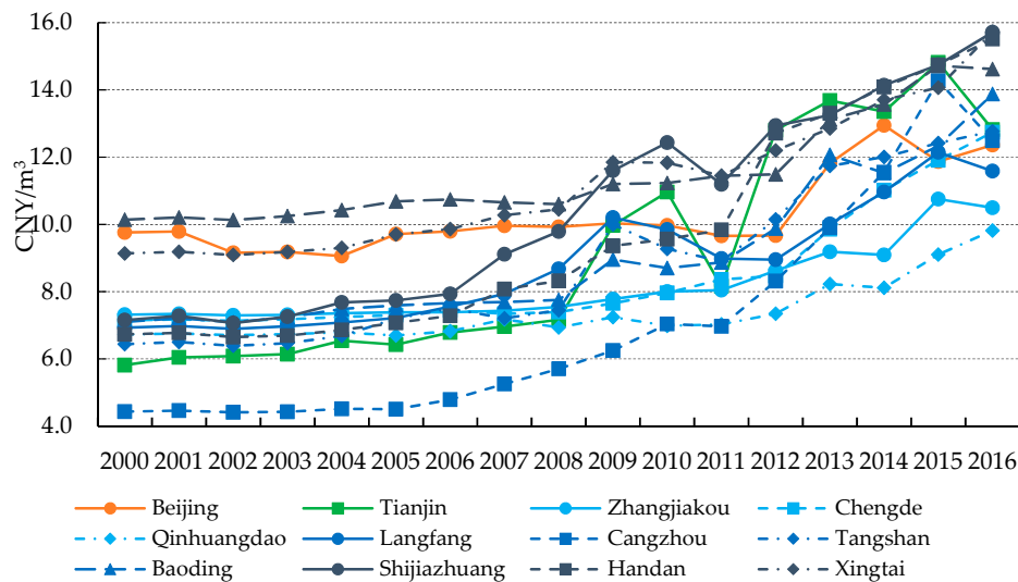
Figure 5. The shadow price of industrial water use in the BTH city region (2000–2016).
