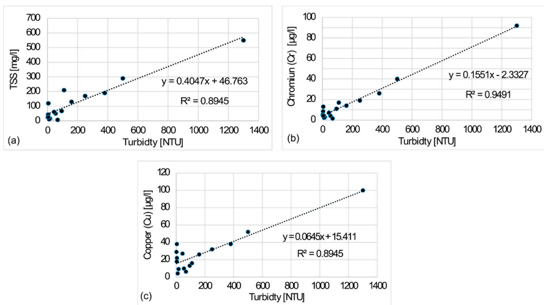
Figure S2. Correlation between turbidity and total suspended solids (a), concentration of chromium (b) and concentration of copper (c).
