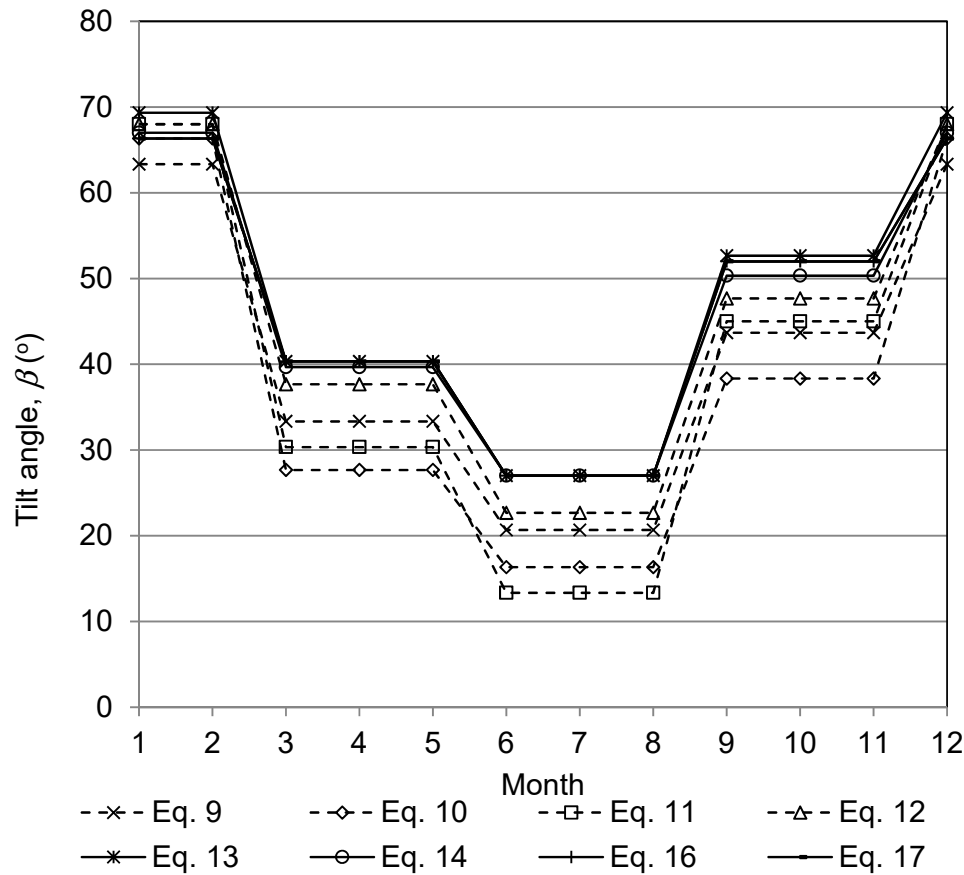
Figure 5. Optimum seasonal tilt angles.
