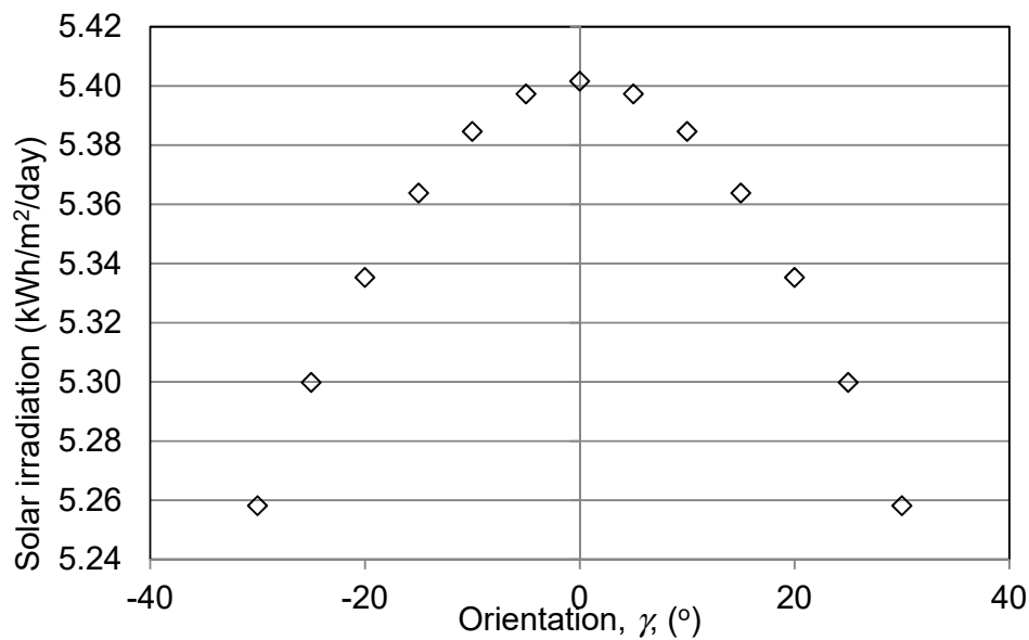
Figure 7. Yearly average solar radiation on a tilted surface for different orientations (Equation (10)).
