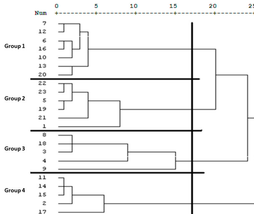
Figure 1. Dendrogram for hierarchical clustering using the Ward's method and the Euclidean distance.
