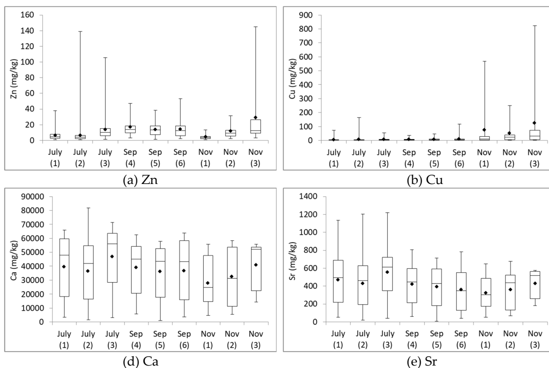
Figure S2. Concentration of metal and trace elements in resins collected during different sampling periods. Note: July (1), July (2), and July (3) denotes three recycling procedures on July 28 th -29 th , August 4 th -5 th , and August 11 th -12 th , respectively; Sep (4), Sep (5), and Sep (6) denotes three recycling procedures on September 30 th , October 7 th , and October 14 th , respectively; Nov (1), Nov (2), and Nov (3) denotes three recycling procedures on November 4 th , 11 th and 18 th , respectively.
