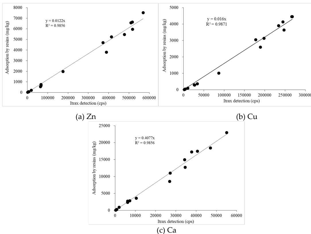
Figure S1. Relationship between resin adsorption and Itrax XRF-CS detection values. Note: cps denotes count per second.
