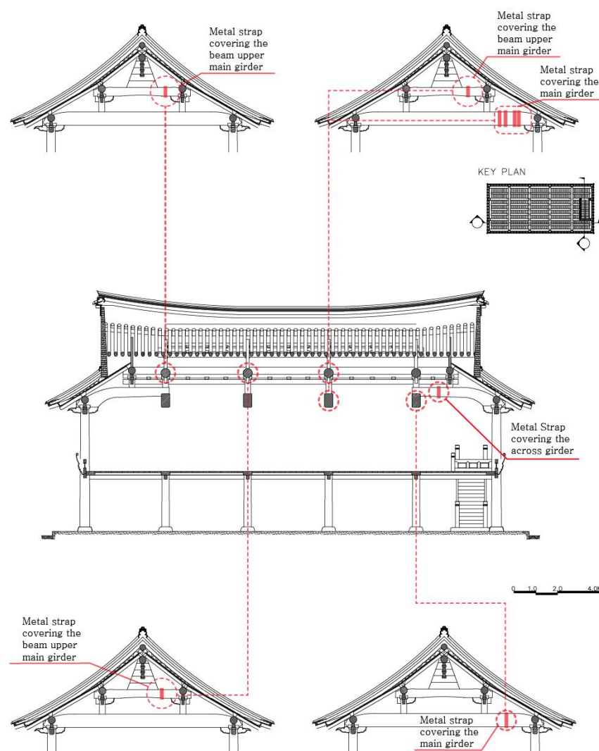
Figure 14. Repaired parts in the main girder and beam upper main girder. (all figures source: author).
