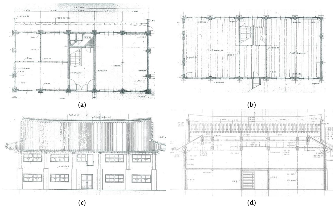
Figure 9. The drawings of Mangseollu before dismantlement in 1999; (a) Drawing of the 1st floor; (b) Drawing of the 2nd floor; (c) The front view; (d) The longitudinal sectional view. (source: National Archives of Korea, author edit).
