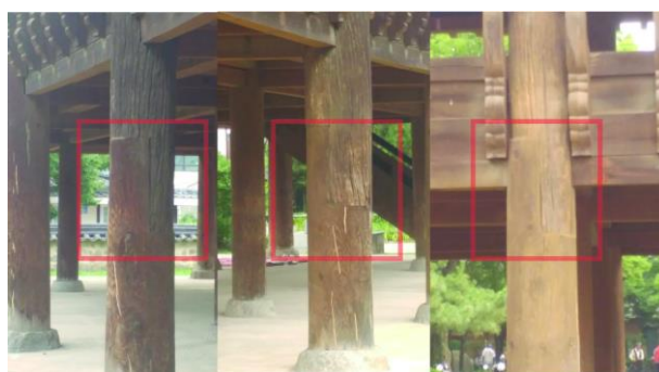
Figure 12. Traces of renovation of the exterior columns on the 1st floor. (all figures source: author).
