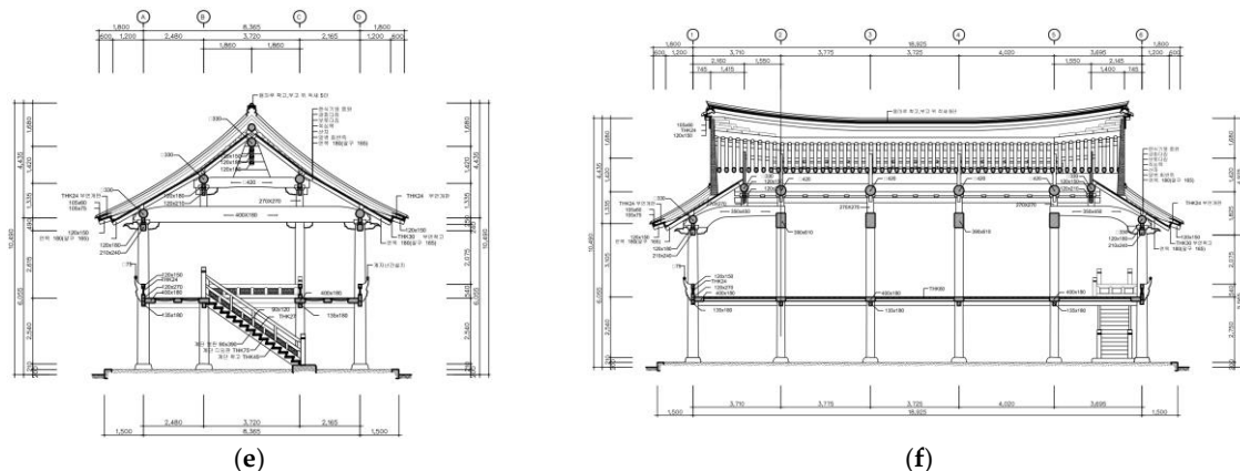
Figure 11. The drawings of present Mangseollu ; (a) Drawing of the 1st floor (Marks indicate the columns with traces of renovation); (b) Drawing of the 2nd floor (Marks indicate the newly added columns); (c) The front view; (d) The lateral view; (e) The longitudinal sectional view; (f) The cross-sectional view. (all figures source: Cheongju Cityhall).
