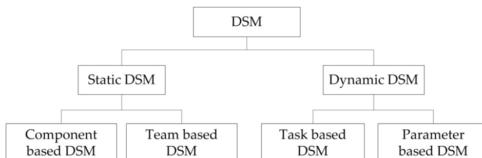
Figure 4. DSM taxonomy.
