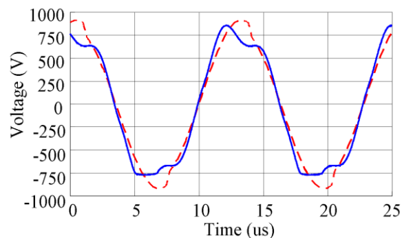
Figure13: Simulated and measured voltage of the transmitter coil. The solid blue line shows the measured result and the dashed red dash line the simulated result.
