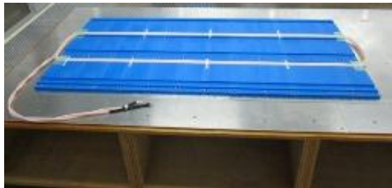
Figure2: Photograph of the measured transmitter coil
