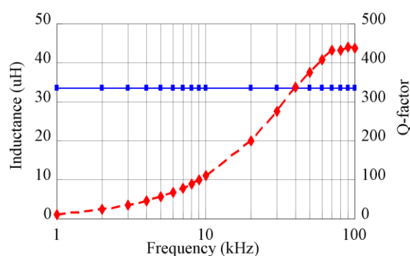
Figure3: Measured inductance and Q-factor of the transmitter coil as a function of frequency. The solid blue line shows the inductance and the dashed red line the Q-factor.
