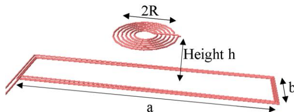
Figure7: Schematic showing the receiver coil positioned above the transmitter coil
