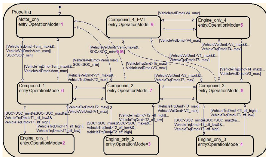
Figure3: Stateflow chart of the energy management controller
