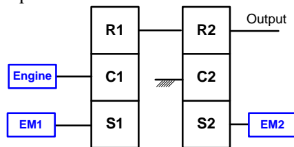
Figure4: Schematic diagram of the benchmark “THS II-like” vehicle
