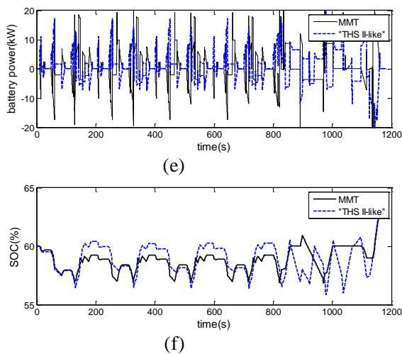
Figure5: Simulation results of NEDC. (a) Vehicle velocity. (b) MMT operation mode. (c) Engine power. (d) Electric machine power. (e) Battery power. (f) Battery SOC.
