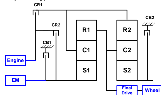
Figure 1: Schematic diagram of the proposed single EM HEV
