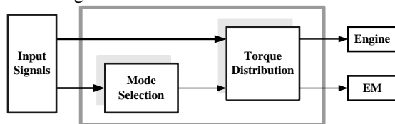
Figure2: Schematic diagram of the proposed single EM HEV
