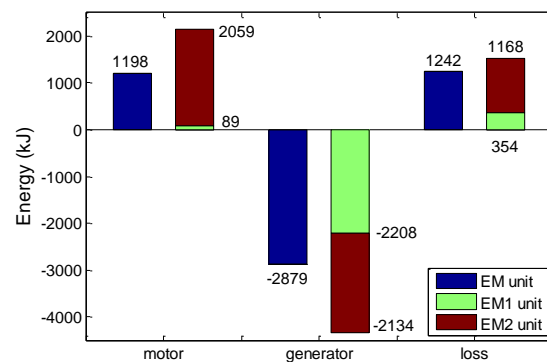
Figure7: Accumulative energy of electric machine units
