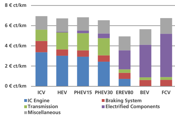
Figure 3: Aggregated distribution of maintenance and repair cost
