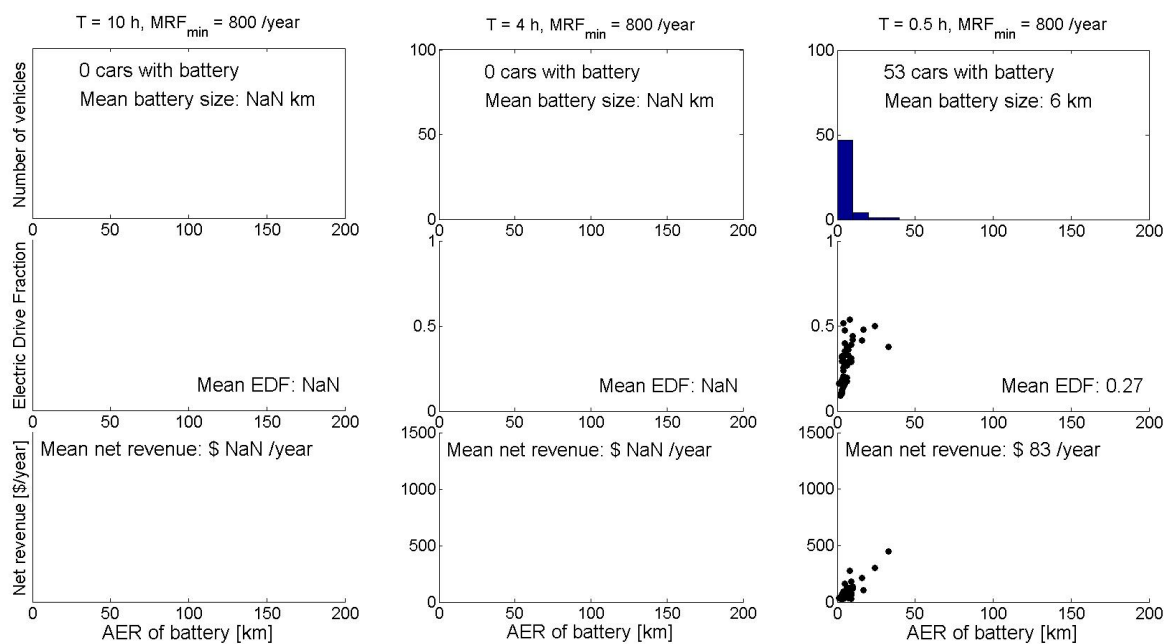
Figure 3: Optimal battery size and the corresponding electric drive fraction and net revenue of cars when MRF_{min} = 800 \text{ yr}^{-1} and the cars can charge at 10, 4 and 0.5 hrs breaks, respectively.
