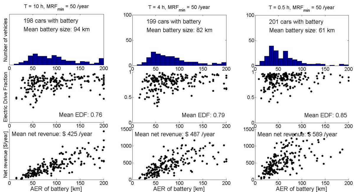
Figure 5: Optimal battery size and the corresponding electric drive fraction and net revenue of cars when MRF_{\min} = 50 \text{ yr}^{-1} and the cars can charge at 10, 4 and 0.5 hrs breaks, respectively.
