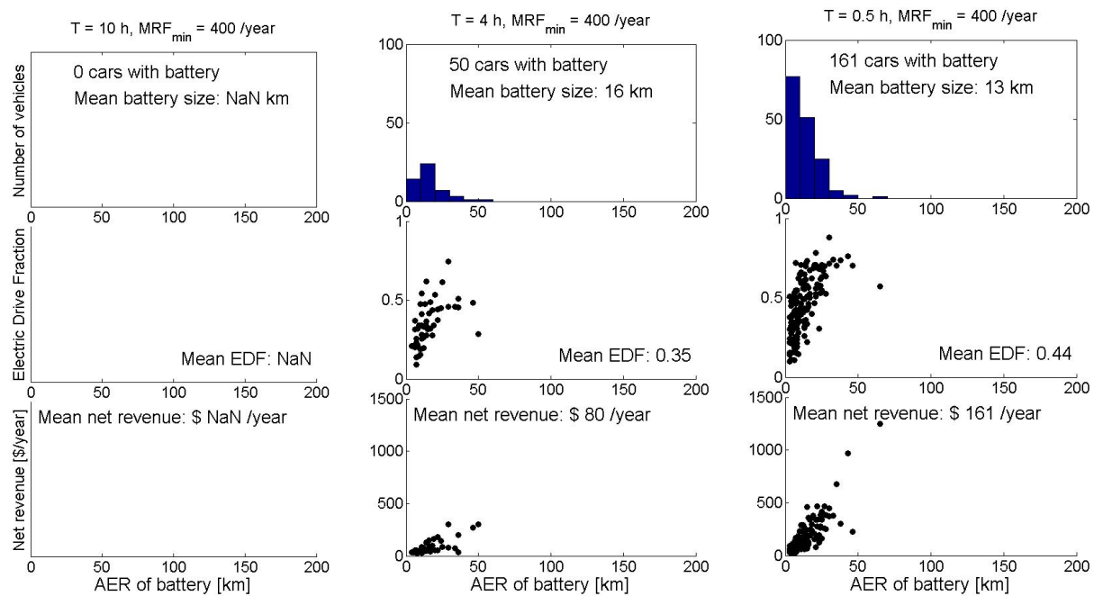
Figure 4: Optimal battery size and the corresponding electric drive fraction and net revenue of cars when MRF_{\min} = 400 \text{ yr}^{-1} and the cars can charge at 10, 4 and 0.5 hrs breaks, respectively.
