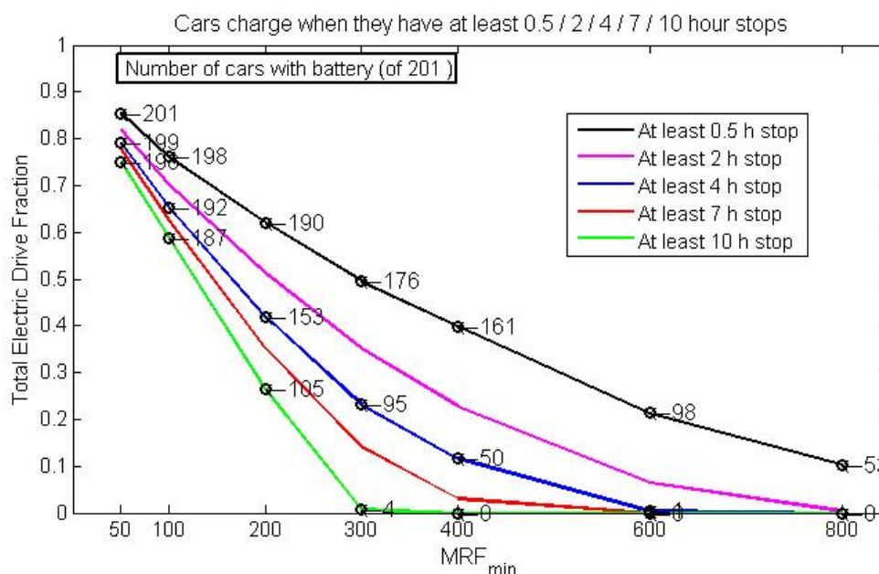
Figure 6: Total fleet electric drive fraction and number of PHEVs of the total fleet of 201 cars in the maximum potential scenario as a function of the viability parameter MRF_{\min} and a range of different minimum break intervals T between 0.5 and 10 hrs.
