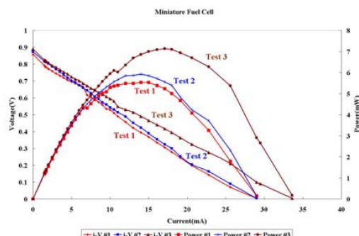
Figure 4: Current-voltage curve and current-power curve of fuel cell performance experiments of micro fuel cell prototype.
