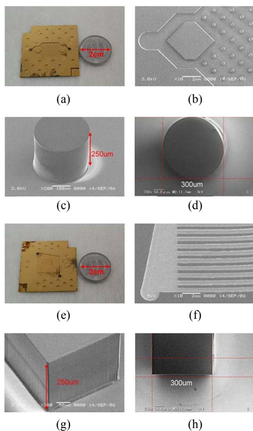
Figure2: Fabricated anode((a)~(d)) and cathode((e)~(h)) channel with Si/SU-8 for micro PEM fuel cell
