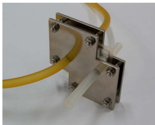
Figure 3: Assembly of micro PEM fuel cell prototype.
