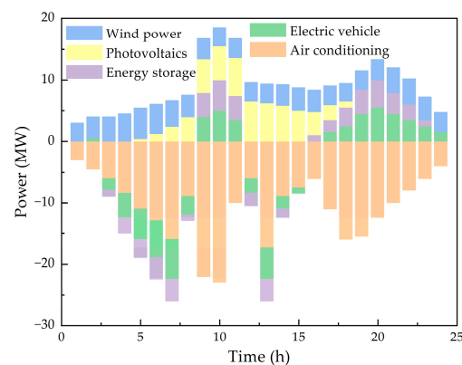
Figure 12. Optimal VPP dispatch result under Scenario 2.
