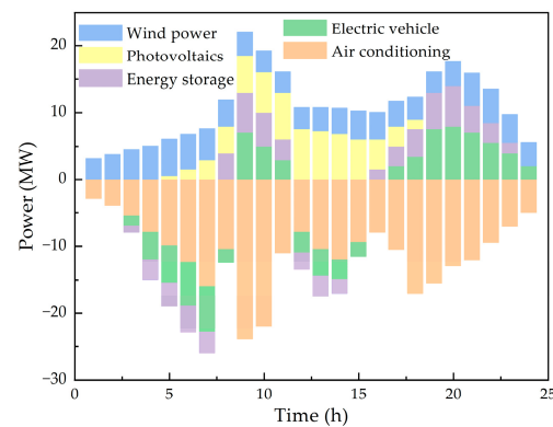
Figure 11. Optimal VPP dispatch result under Scenario 1.
