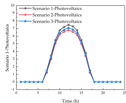
Figure 15. Comparison of photovoltaic accommodation under three scenarios.
