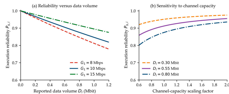
Figure 21. Analytical behavior of the execution-reliability model.
