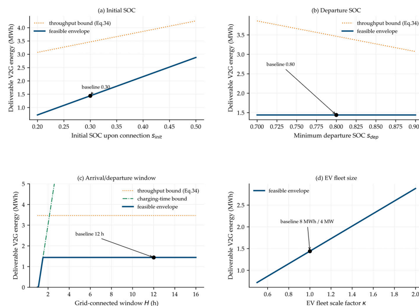
Figure 24. Maximum daily deliverable V2G energy envelope.
