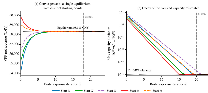
Figure 20. Multi-start verification of the coupled Nash–Stackelberg equilibrium.
