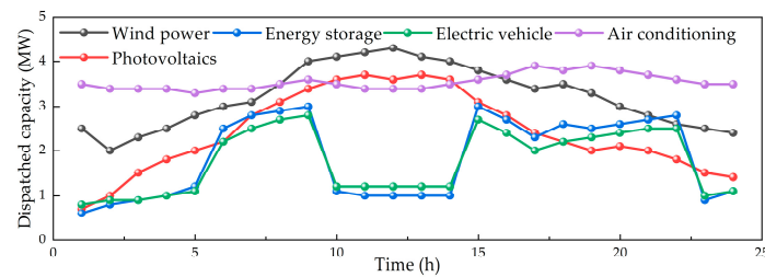
Figure 7. Capacity-layer dispatched capacity of each resource agent under Scenario 1.
