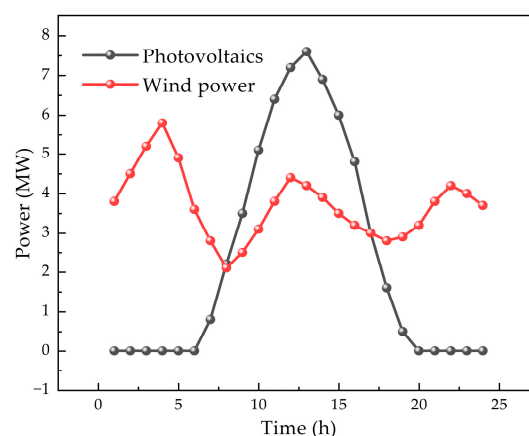
Figure 2. Predicted wind and photovoltaic output.
