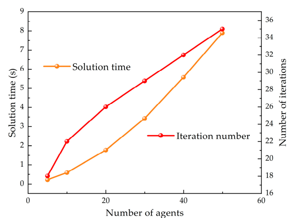
Figure 18. Influence of agent number on solution time and iteration times.
