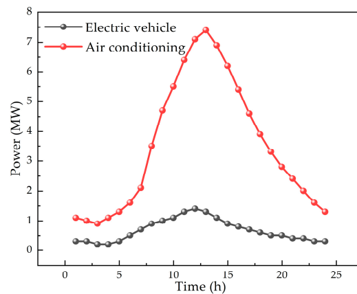
Figure 3. Predicted electric vehicle and air-conditioning load profiles.
