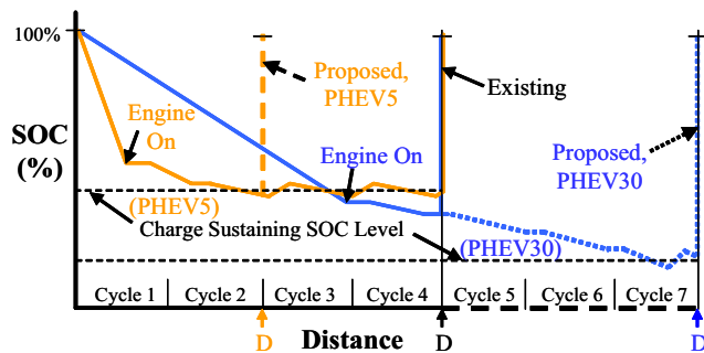
Fig. 5 Hypothetical FCT SOC profiles for two example PHEVs over a UDSS cycle test
