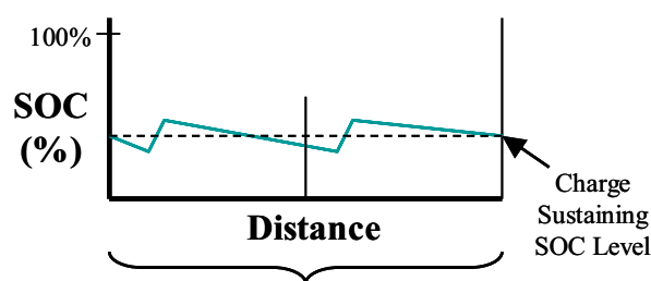
Fig. 2 PCT to measure Charge-Sustaining (CS) vehicle fuel economy; illustrated with application to the UDDS or HWFET test cycles
