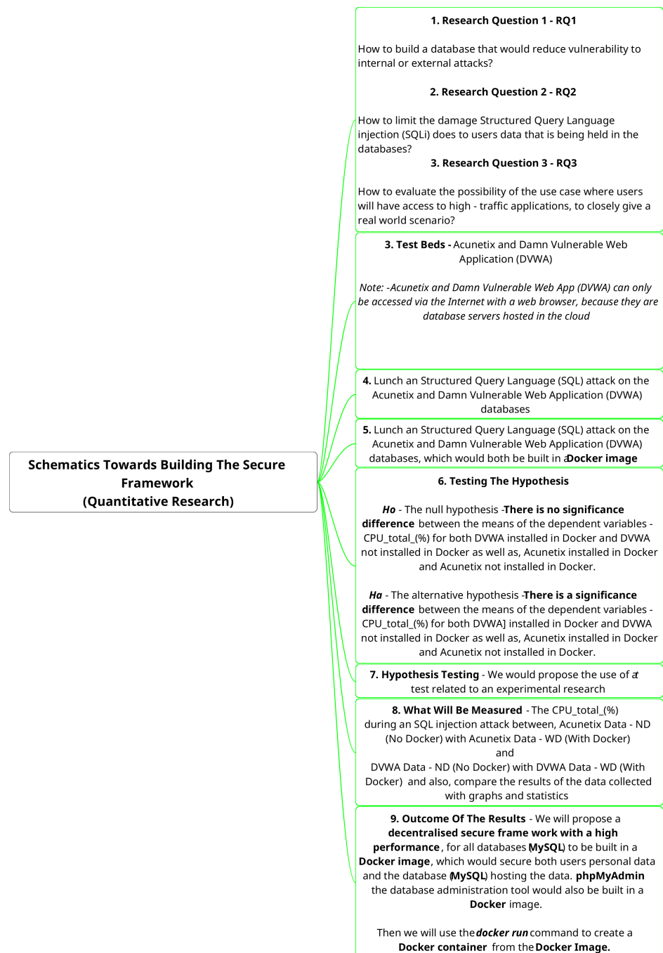
Figure 3. Schematics towards building the secure framework (quantitative research).
