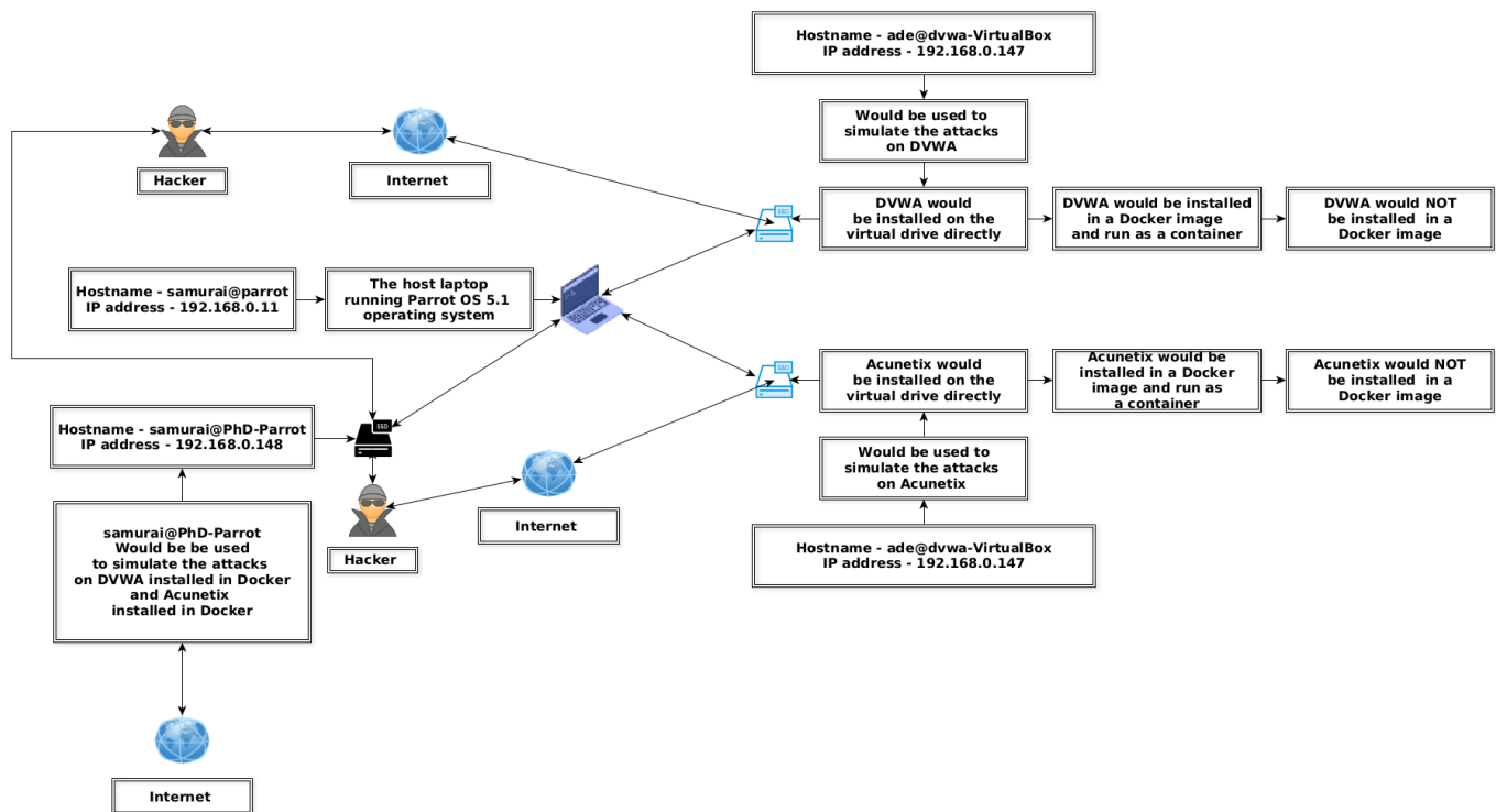
Figure 2. Schematic diagram of the laboratory. Note: all IP addresses in Figure 2 are unique addresses that identify a device on the local network.
