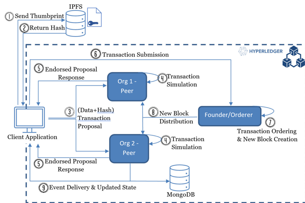
Figure 1. Architecture design.
