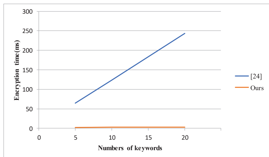
Figure 4. The encryption times of ours and [24].
