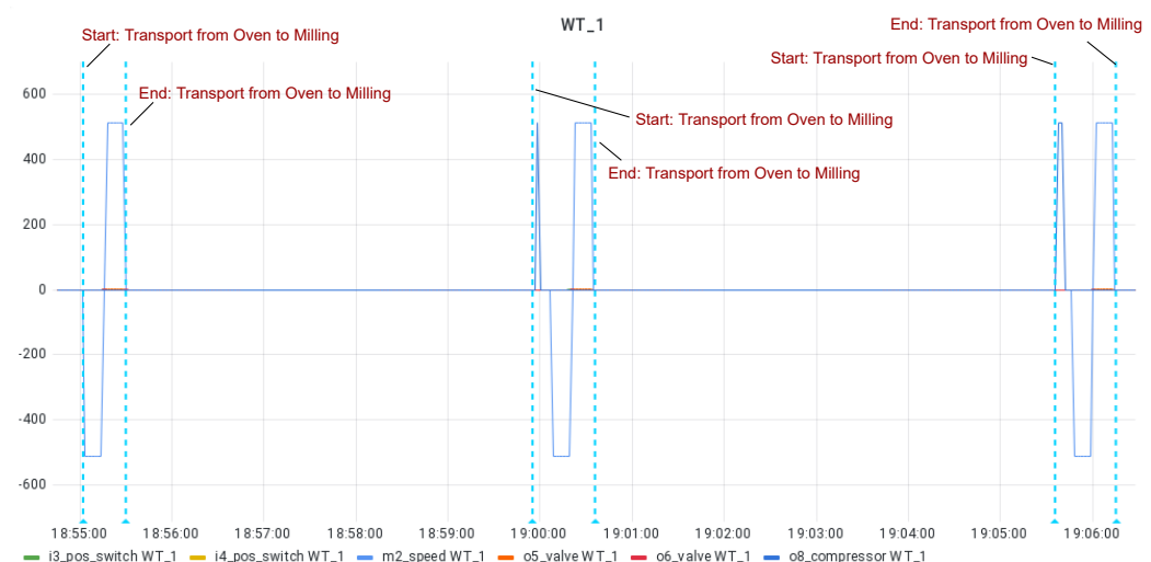
Figure 10. Details of the IoT data filtered by the WT_1 component with manual annotations.
