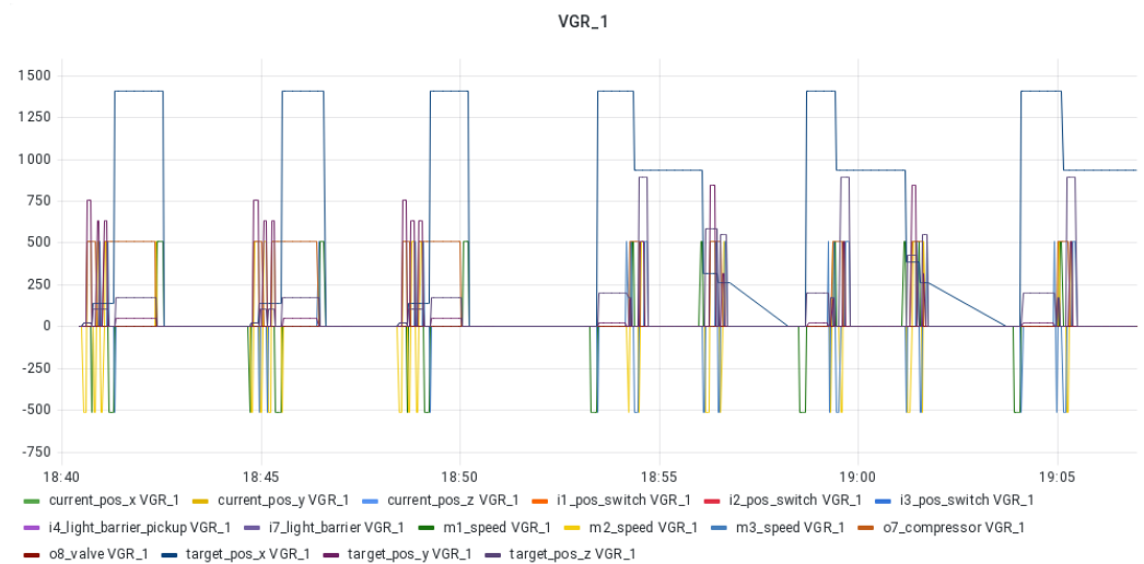
Figure 8. IoT data filtered by the VGR_1 (Vacuum Gripper Robot) component.
