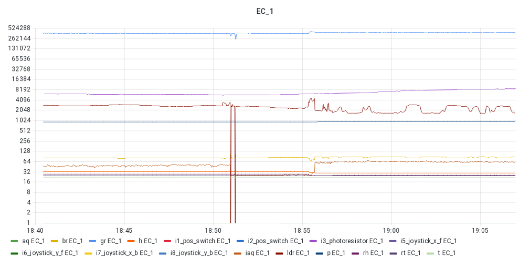
Figure 9. IoT data filtered by the EC_1 (Environment and Camera) component.
