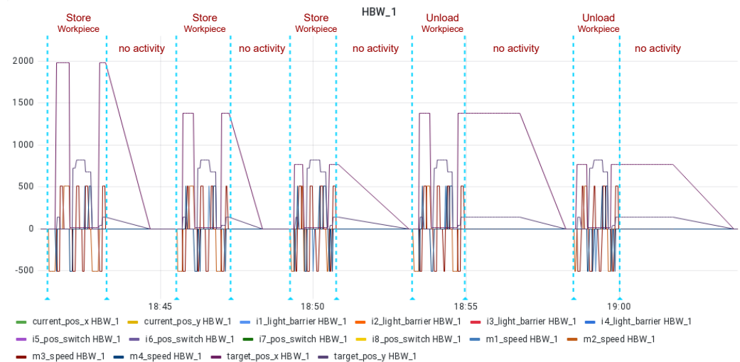
Figure 16. Similar activities found for HBW_1 component.
