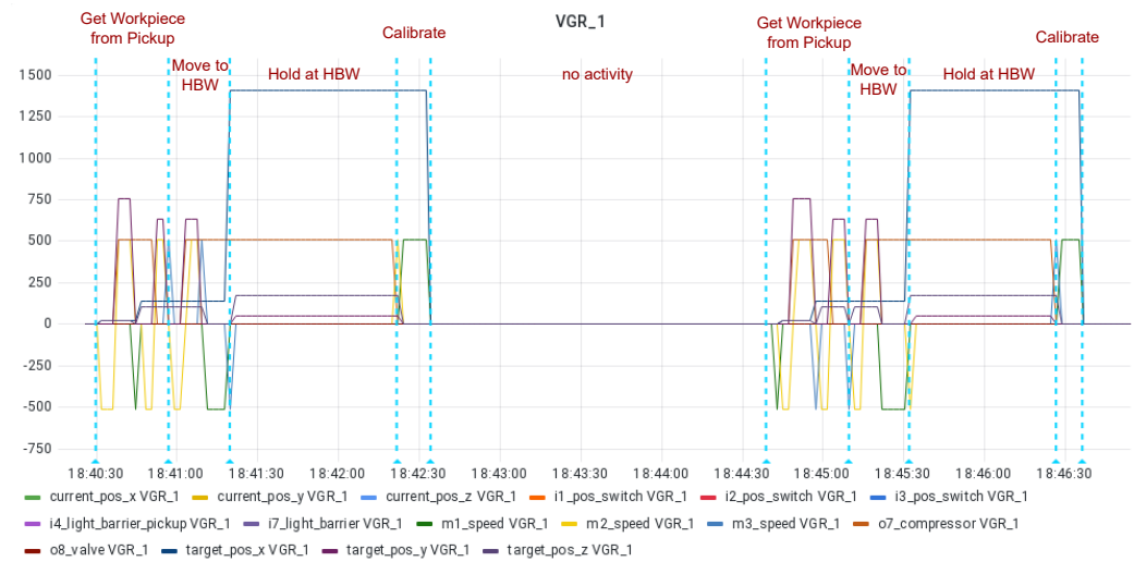
Figure 15. Similar activities found for VGR_1 component.
