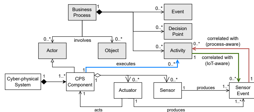
Figure 1. UML class diagram of BPM–CPS concepts serving as basis for our work (adapted from [5]).
