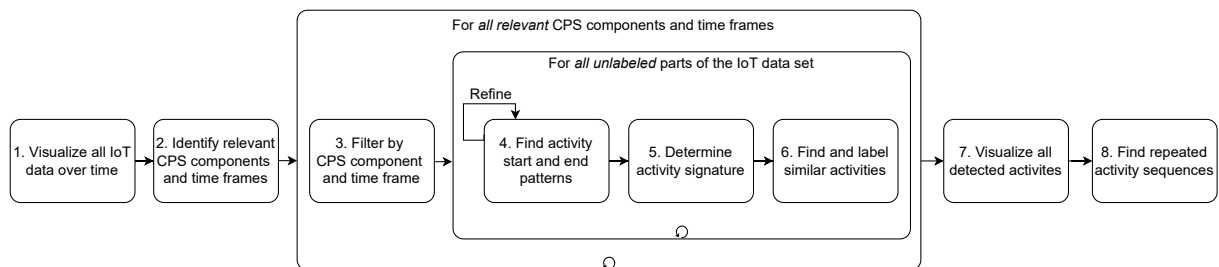
Figure 18. Derived method for detecting activity executions from IoT data.
