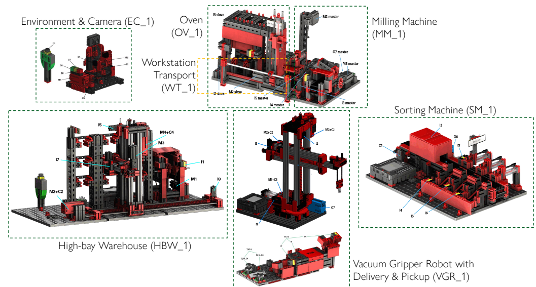
Figure 2. Components and layout of the smart factory model, partially adapted from [22] with permission.
