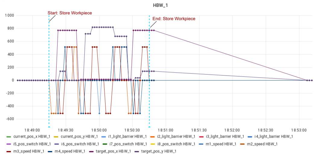
Figure 11. Details of a part of IoT data filtered by the HBW_1 component with annotations.
