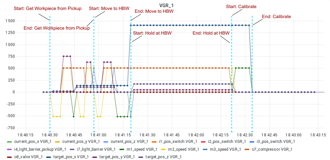
Figure 12. First part of IoT data filtered by the VGR_1 component with manual annotations.
