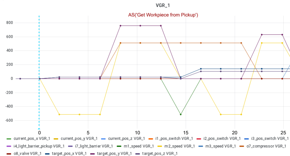
Figure 14. Activity Signature for Get Workpiece from Pickup executed by VGR_1.
