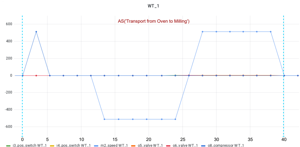
Figure 13. Activity Signature for Transport from Oven to Milling executed by WT_1.
