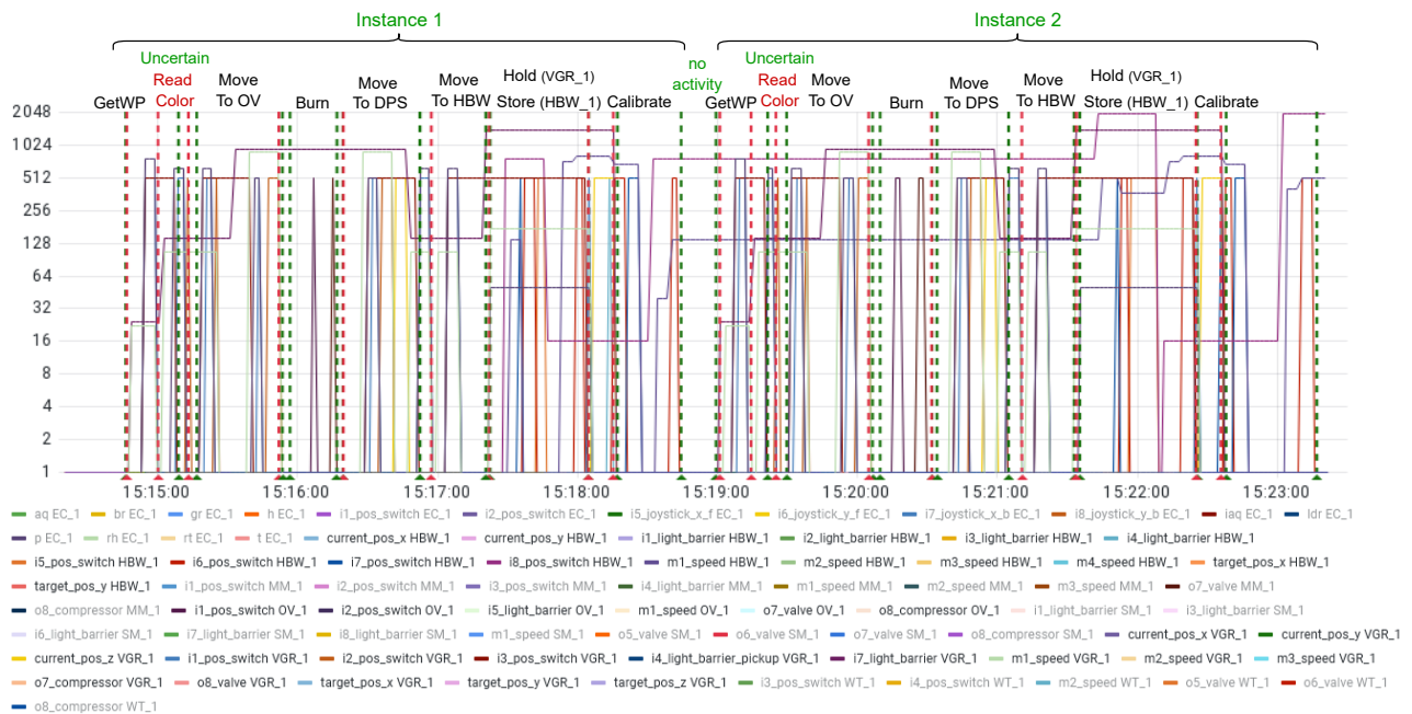
Figure 21. Evaluation IoT data set labeled by the analyst (green), BPM system (red) or both (black).
