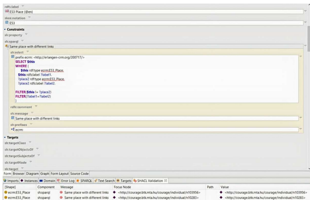
Figure 14. Validating same places with different URIs.
