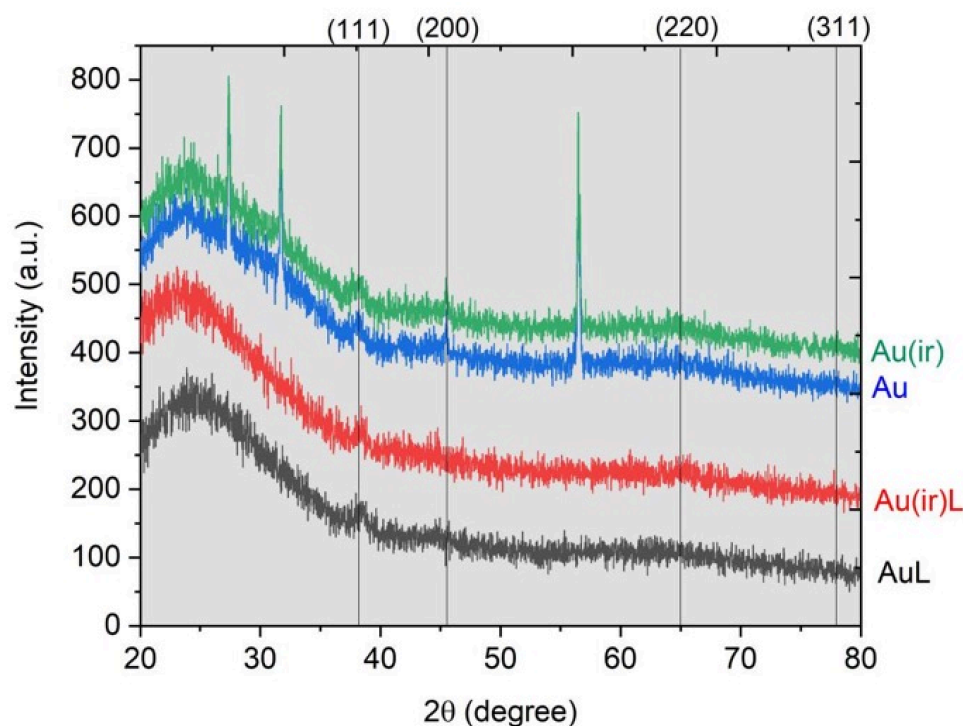
Figure 3. Diffractograms of the Au, Au(ir), AuL, and Au(ir)L samples.
