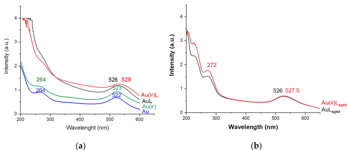
Figure 2. Spectrophotometric analysis of the (a) Au, Au(ir), AuL and Au(ir)L, and (b) of Au(ir)L aged and AuL aged samples.
