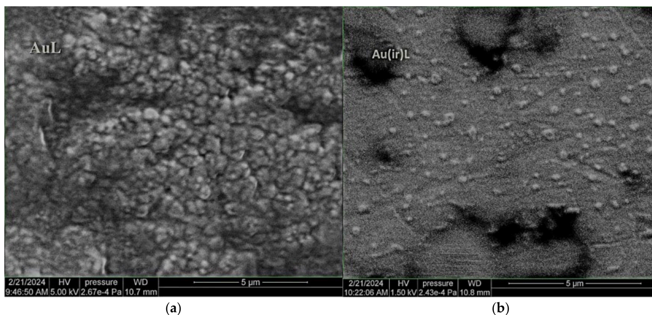
Figure 11. SEM images of the AuL (a) and Au(ir)L (b) samples.
