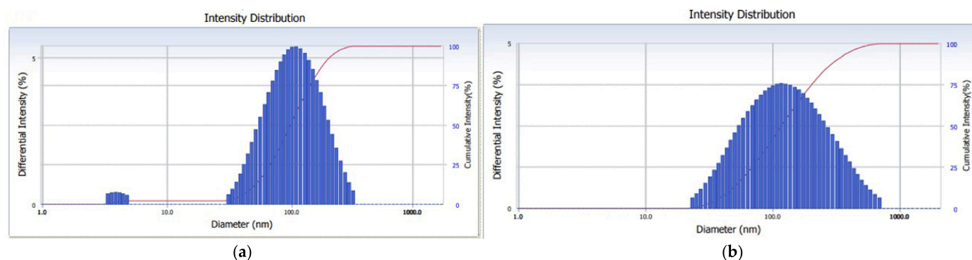
Figure 7. Dimensional histograms of the AuL (a) and Au(ir)L (b) samples. The red curve represents the Cumulative Intensity distribution (%).
