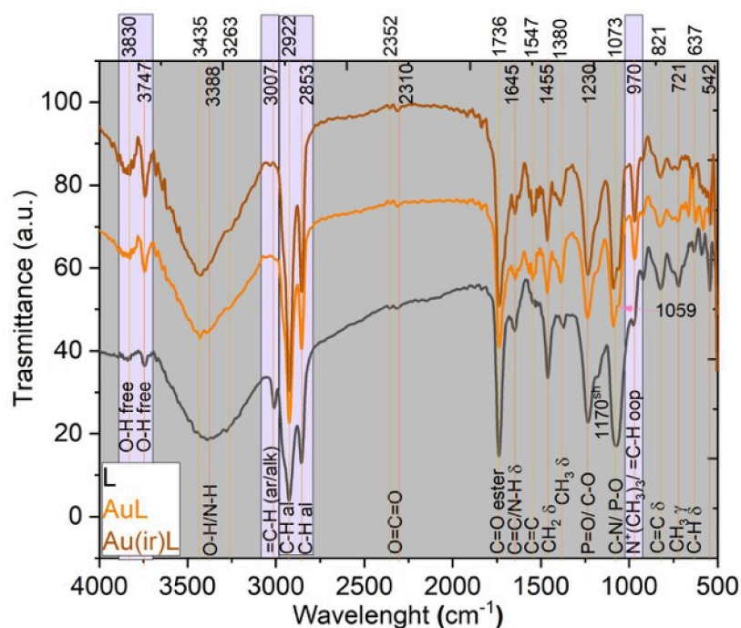
Figure 8. FTIR spectra of phosphatidylcholine—lipid (L), AuL, and Au(ir)L samples.
