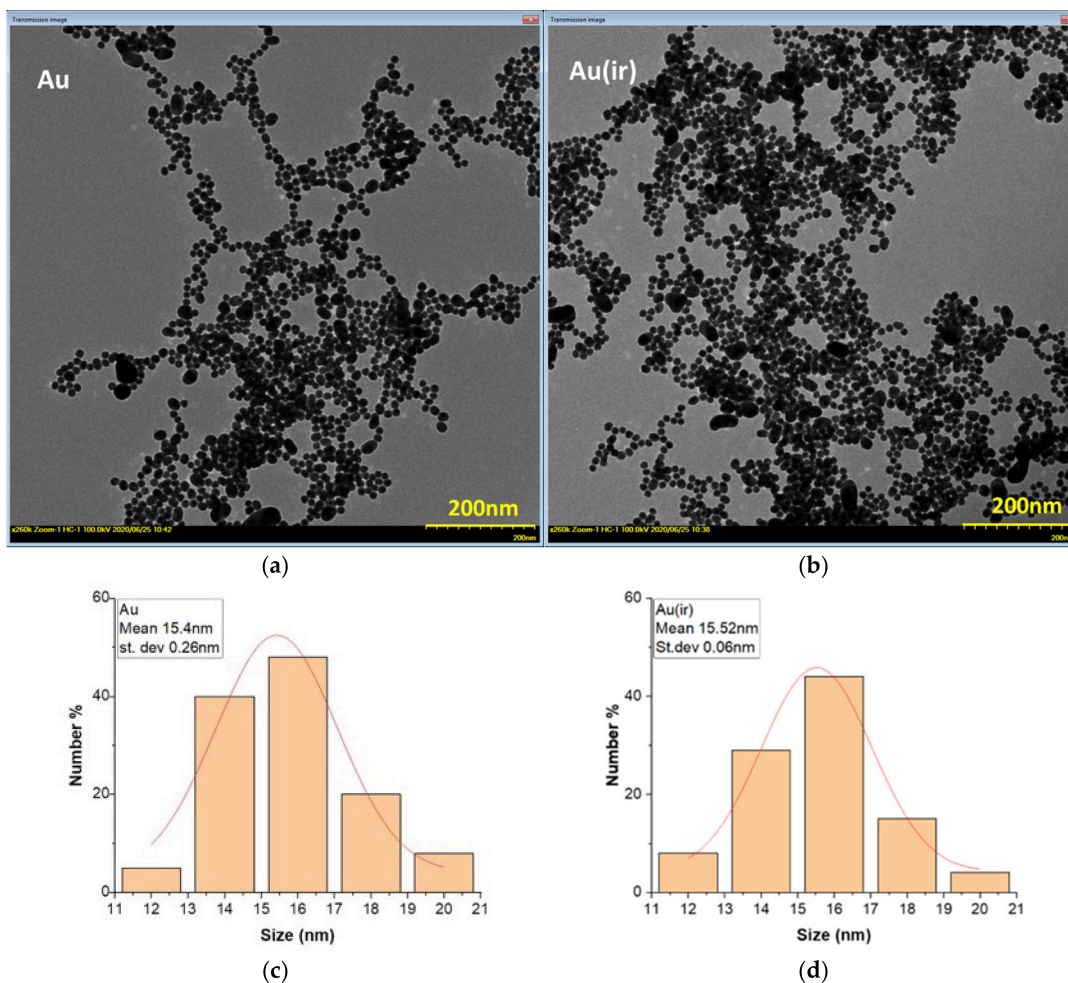
Figure 4. TEM images of the Au sample (a) and Au(ir) sample (b) and the histograms of the dimensional distributions of the Au sample (c) and the Au(ir) sample (d). The red line represents the fitting of the distribution graphics.
