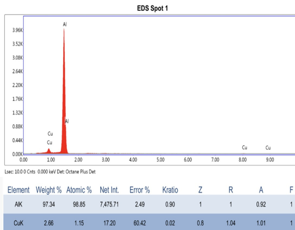
Figure 10. EDX spectrum of the aluminum substrate.
