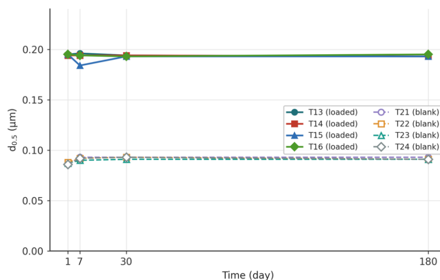
Figure 3. Particle size ( d_{0.5} ) of resveratrol-loaded (T13–T16, solid lines/filled symbols) and unloaded (T21–T24, dashed lines/open symbols) ethosomes over 180 days at 25 \pm 2^\circ\text{C} ; d_{0.5} , volume-weighted median diameter.
