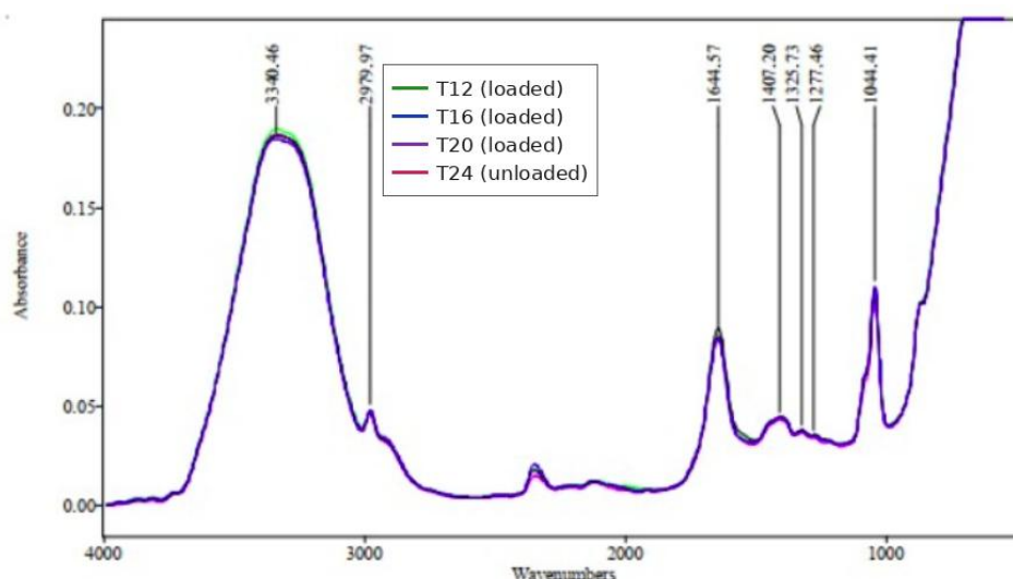
Figure 7. Comparative FT-IR spectra of the unloaded ethosome (T24) and the resveratrol-loaded ethosomes (T12, T16, T20). The spectra are essentially superimposable, showing phospholipid-dominated band patterns and no new covalent bands upon resveratrol loading. FT-IR, Fourier-transform infrared spectroscopy.
