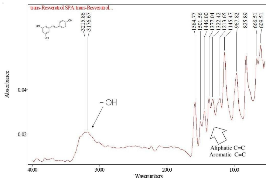
Figure 1. FT-IR, Fourier-transform infrared spectroscopy. FT-IR spectrum of trans-resveratrol showing the characteristic O–H and aromatic/aliphatic C=C absorption bands.
