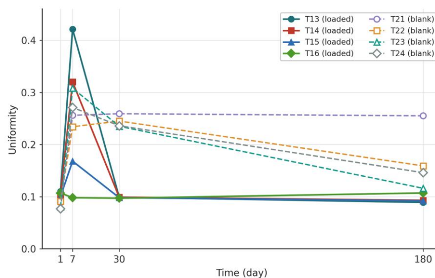
Figure 4. Size distribution uniformity of resveratrol-loaded (T13–T16, solid lines/filled symbols) and unloaded (T21–T24, dashed lines/open symbols) ethosomes over 180 days.
