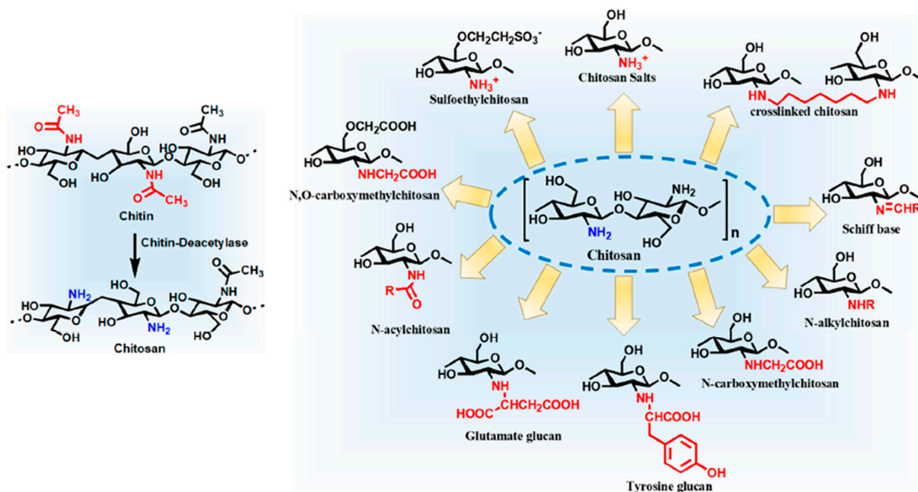
Figure 2. Functionalized chitosan derivatives. Adapted from reference [88].
