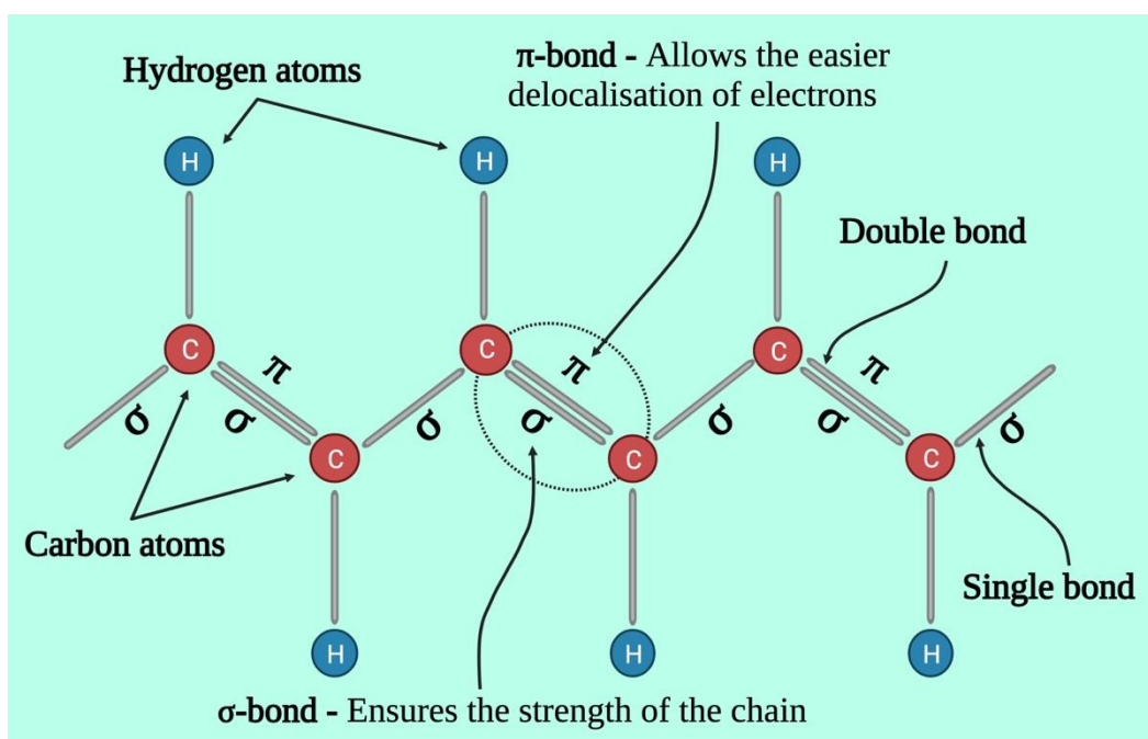
Figure 2. Structural representation of conductive polymer backbone.
