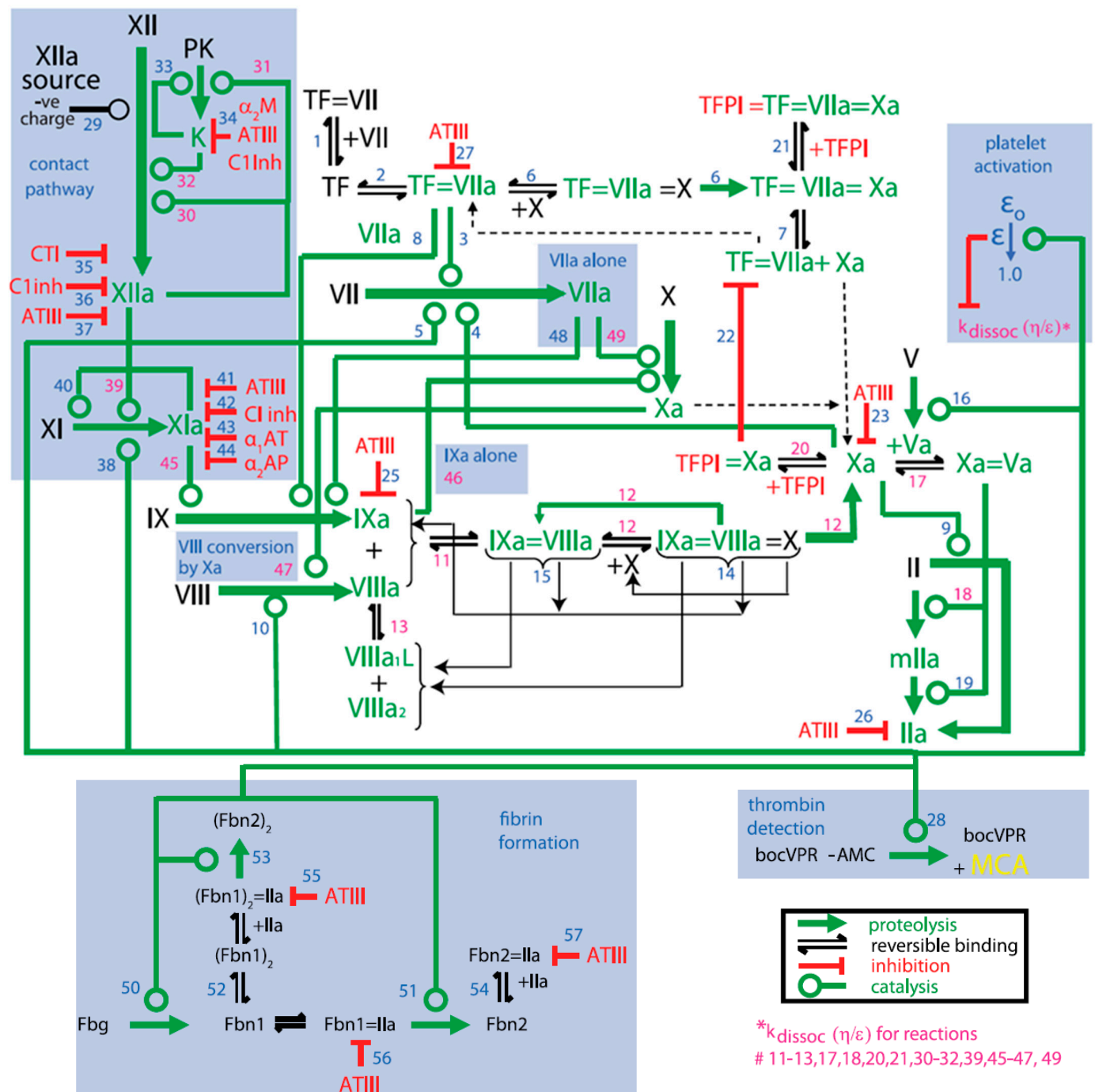
Figure 3. Schematic of the Platelet–Plasma dynamics from the Chatterjee model [5]. Blue highlighted portions represent additions to the Hockin–Mann model [2]. Alpha-1 antitrypsin (α1AT); alpha-2 antitrypsin (α2AT); alpha-2-macroglobulin (α2M); antithrombin-III (ATIII); C1-inhibitor (C1Inh); corn trypsin inhibitor (CTI); fibrin I (Fbn1); fibrin II (Fbn2); fibrinogen (Fbg); kallikrein (K); meizothrombin (mIIa); platelet activation factor (ε); prekallikrein (PK); tissue factor (TF); prothrombin (II); thrombin (IIa); tissue factor pathway inhibitor (TFPI). Blue numbers are the reaction steps in the model and pink numbers are those reactions whose dissociation rate constant is modified by the platelet activation factor (ε).
