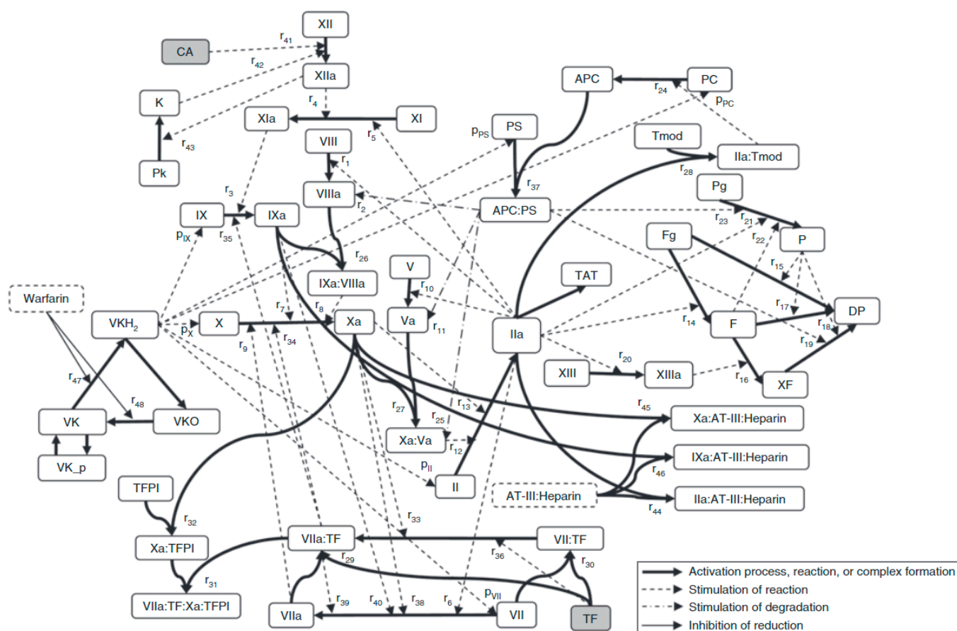
Figure 4. The scheme of the coagulation network model from the Wajima model [6]. The bold solid lines represent the activation process, complex formation, reduction, or oxidization; the broken lines represent stimulation of reaction or production; the dot-bar lines represent stimulation of degradation; the solid lines represent inhibition of reduction. Activated protein C (APC); antithrombin-III (AT-III); activator for the contact system (CA); degradation product (DP); fibrin (F); fibrinogen (Fg); prothrombin (II); thrombin (IIa); prekallikrein (Pk); kallikrein (K); plasmin (P); protein C (PC); plasminogen (Pg); protein S (PS); thrombin–antithrombin complex (TAT); tissue factor (TF); tissue factor pathway inhibitor (TFPI); thrombomodulin (Tmod); vitamin K (VK); vitamin K hydroquinone (VKH2); vitamin K epoxide (VKO); cross-linked fibrin (XF). See original publication [6] for more details on species and reactions.
